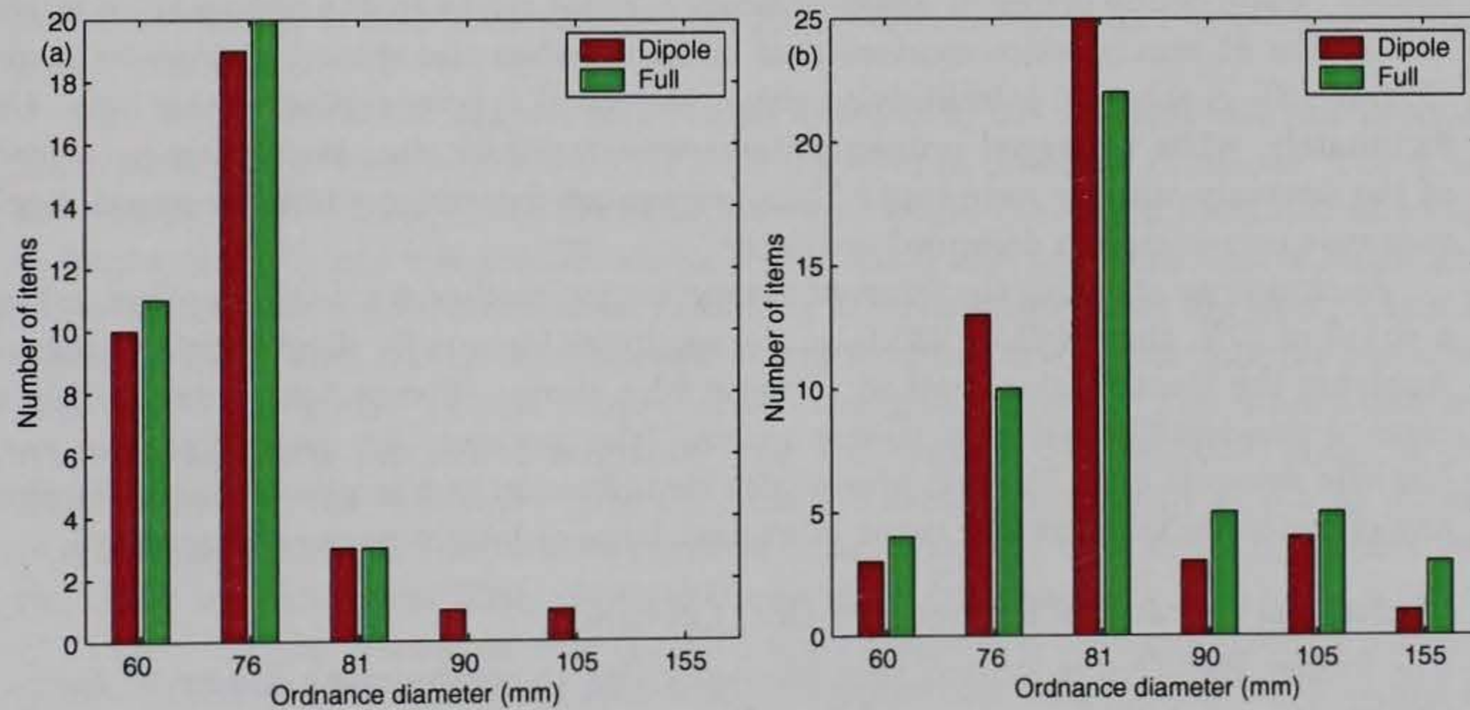
Figure 12: Identification results for the Guthrie Road data using both the dipole and dipole plus octupole methods for (a) 76-mm projectiles; and (b) 81-mm mortars.
