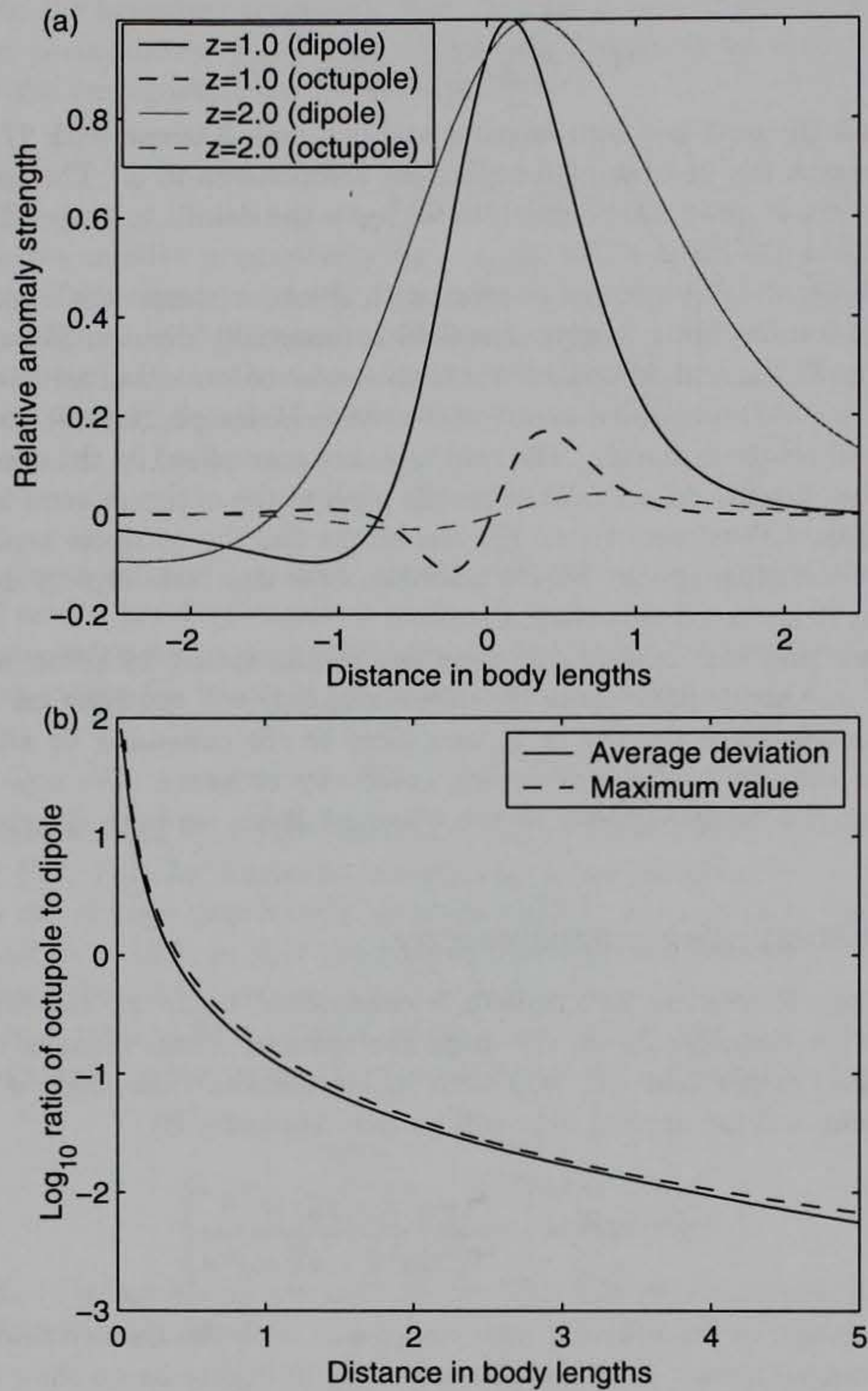
Figure 2: (a) Dipole and octupole terms at one and two body lengths distance; (b) \text{Log}_{10} of the ratio of the octupole to dipole terms for a 105-mm projectile at 45^\circ inclination
