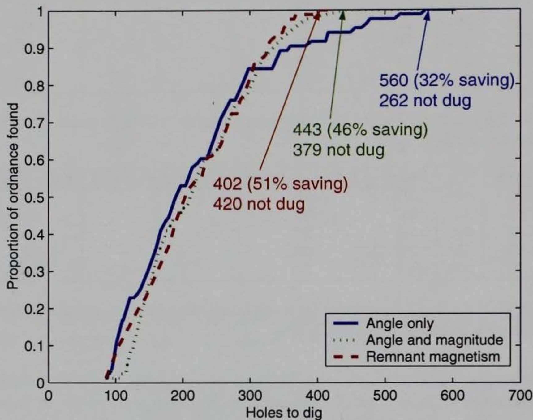
Figure 10: Yield of ordnance with number of holes dug for the three discrimination methods. For all methods it is assumed the 85 anomalies with poor fits are excavated first.
