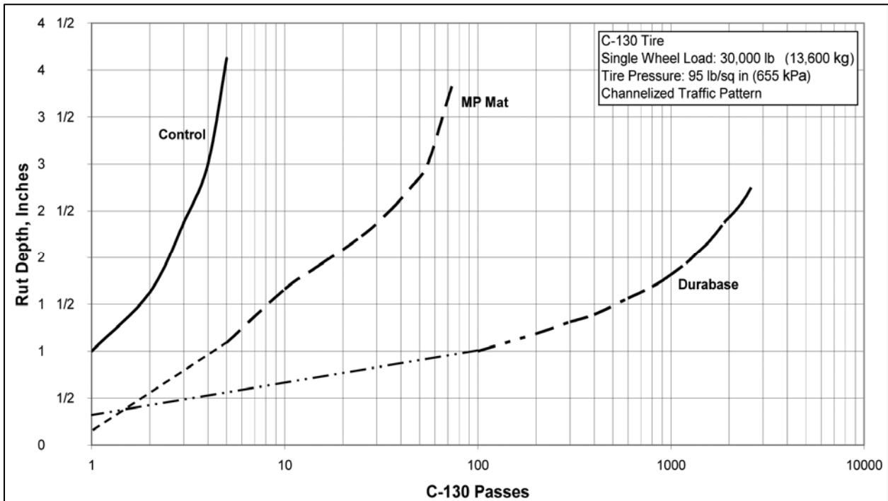
Figure 6. Rut depth for low-strength subgrade (3 to 5 CBR) test items
