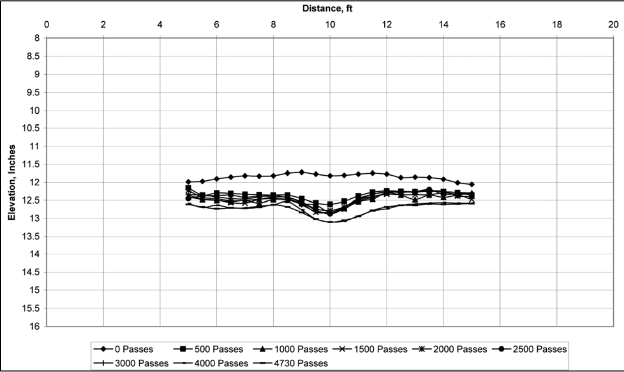
Figure 9. Permanent surface deformation cross section for DURA-BASE on high-strength subgrade (40 to 50 CBR)
