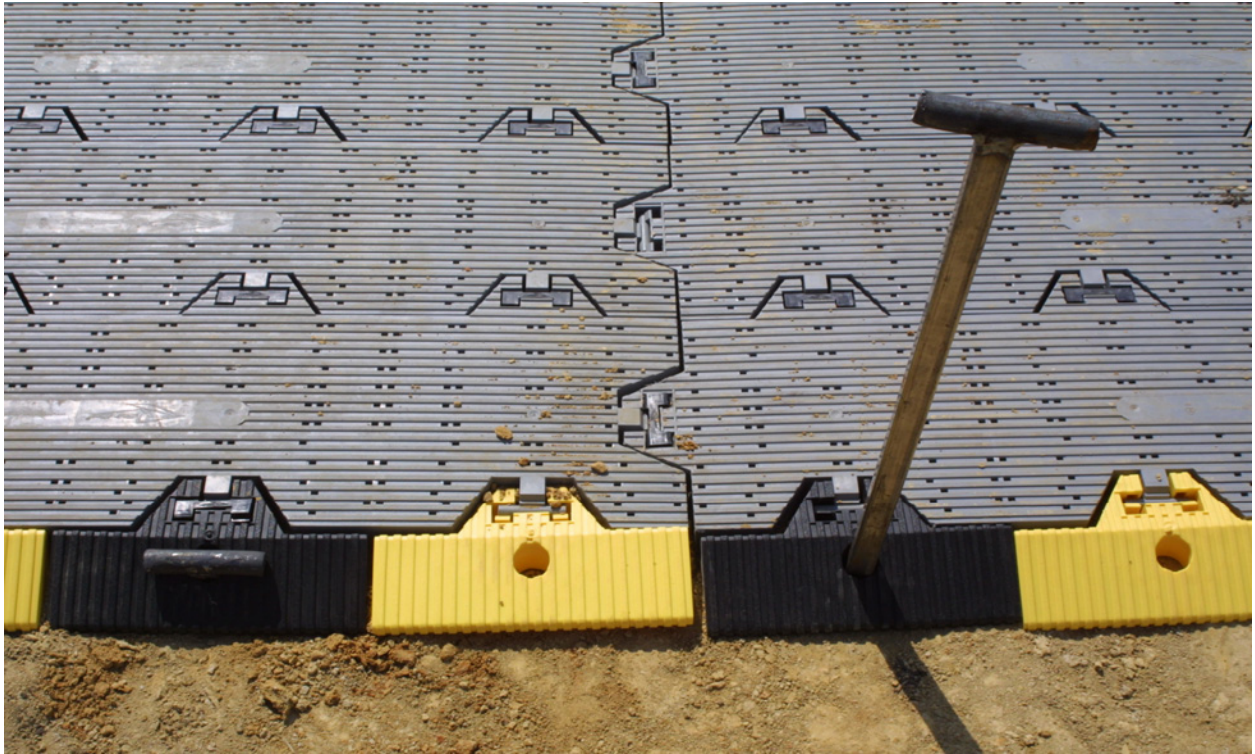
Photo 14. SUPA-TRAC with edge pieces and pins used to tie down the edges
