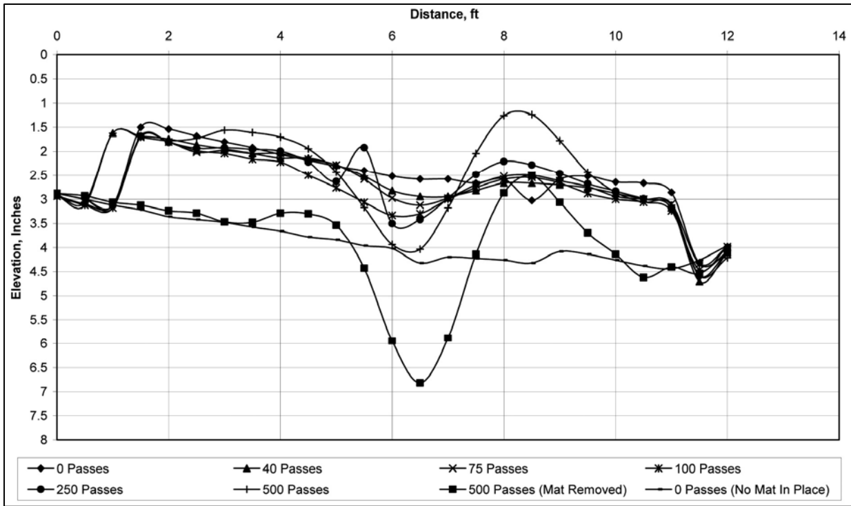
Figure 12. Permanent surface deformation cross section for Rolla Road on high-strength subgrade (40 to 50 CBR)
