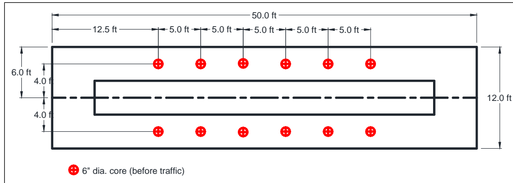
Figure 74. Layout for post construction coring of each test item.
