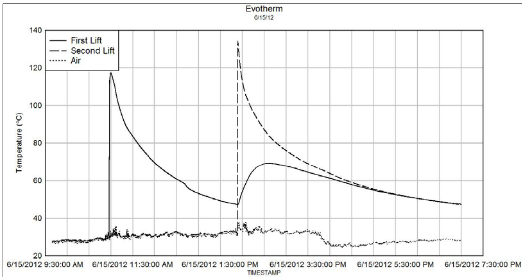
Figure 73. Temperature of Evotherrm™ WMA pavement during construction.
