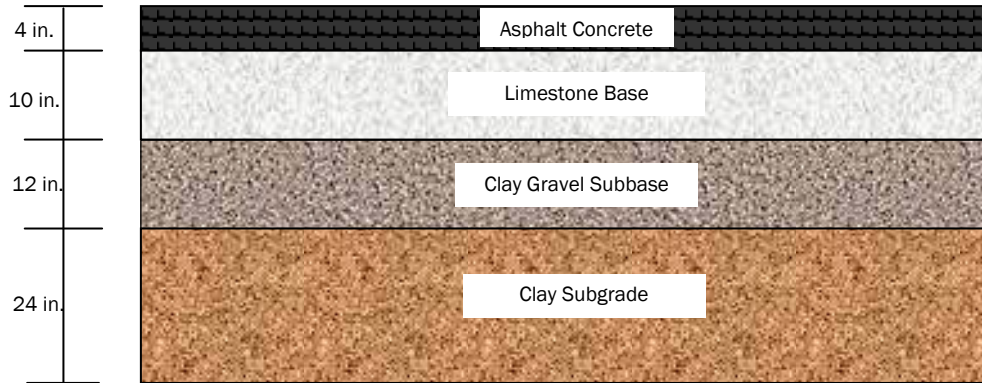
Figure 3. Pavement structure of the test items.
