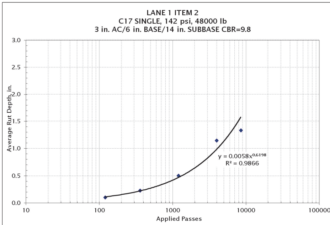
Figure 58. Rutting development on Lane 1 Item 2.
