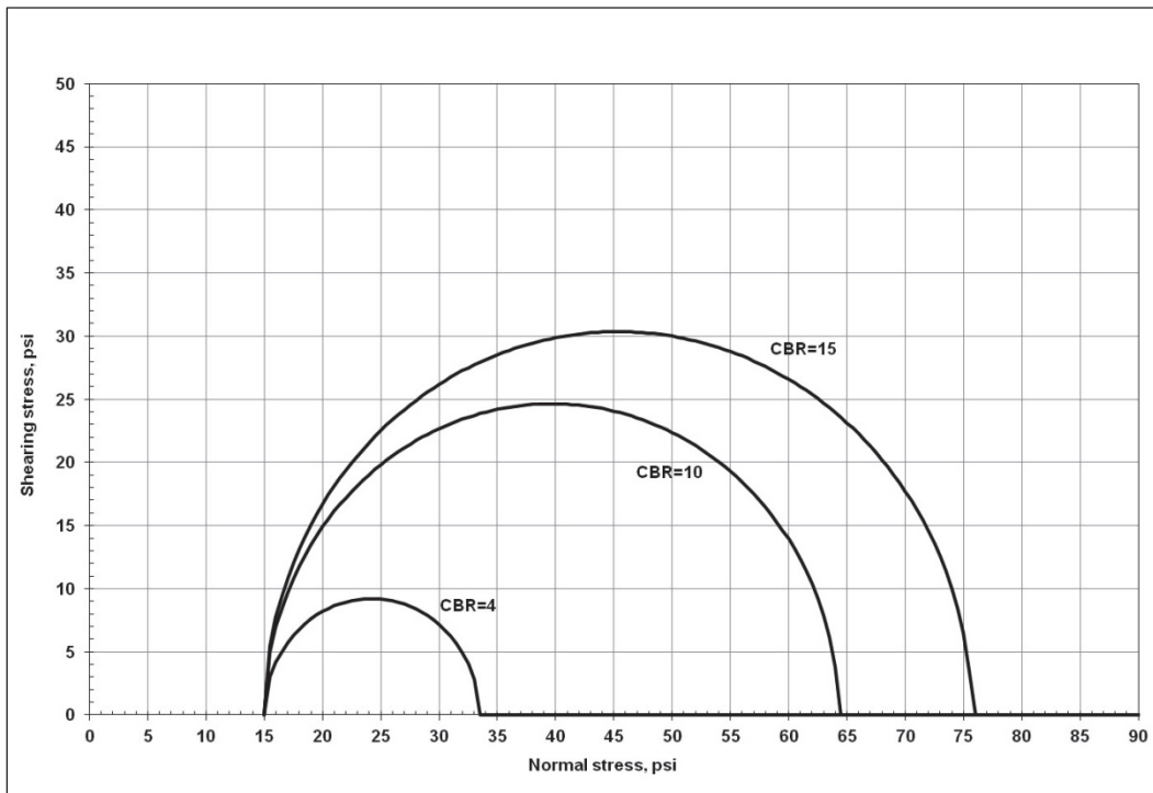
Figure 11. Subgrade material Mohr circles at different CBR values.
