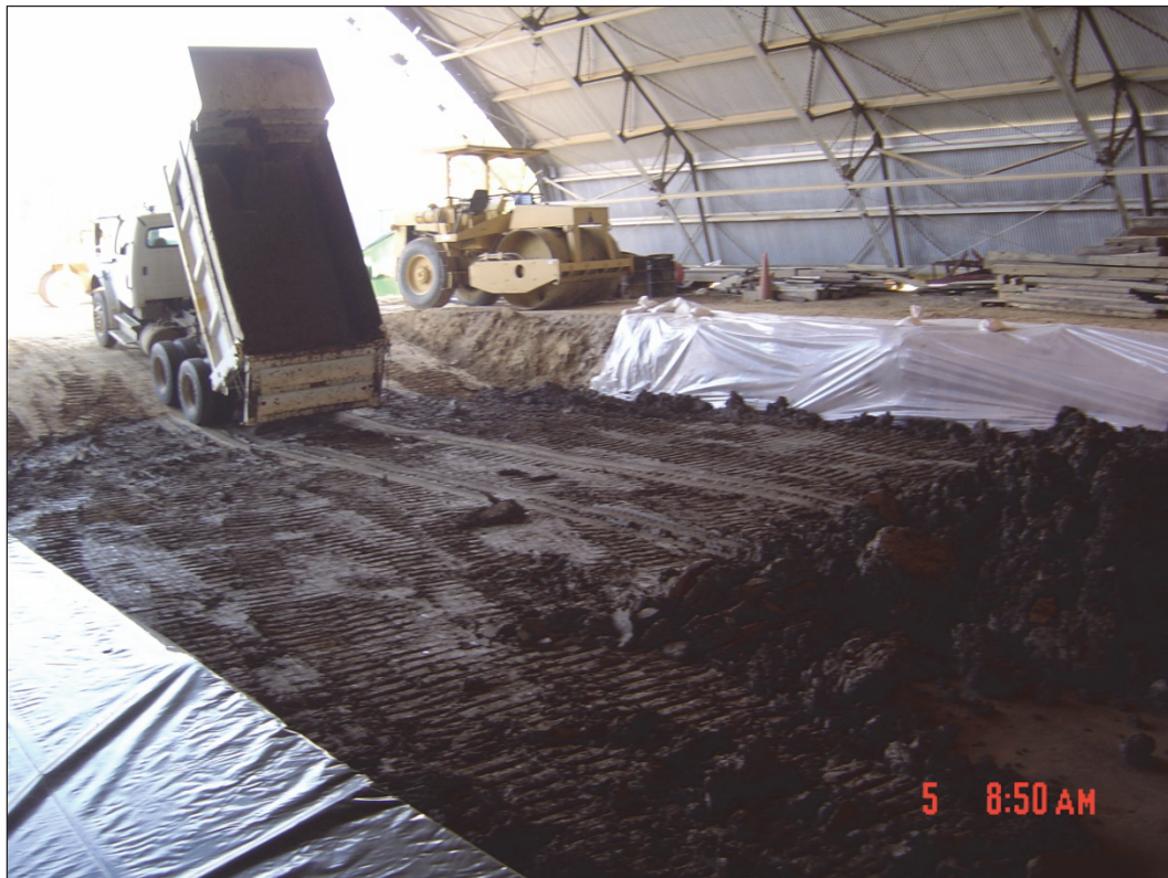
Figure 21. Subgrade material placement.
