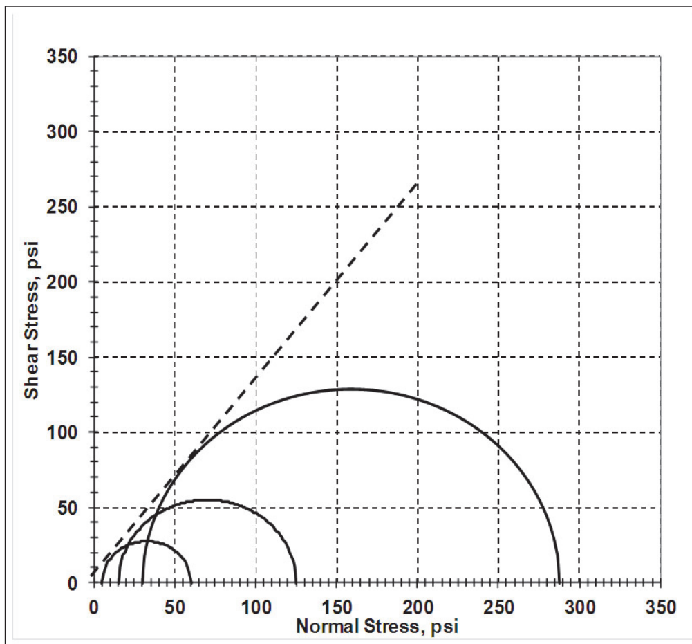
Figure 15. Base course material Mohr's circles.
