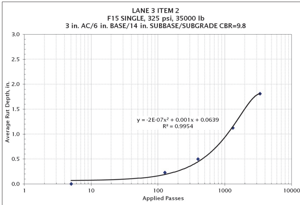
Figure 62. Rutting development on Lane 3 Item 2
