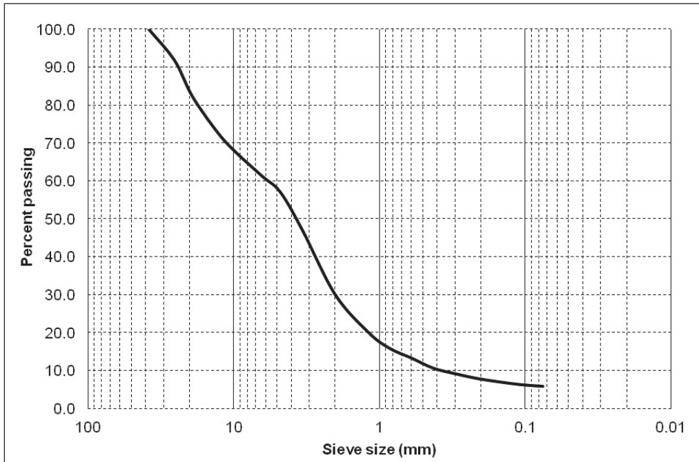
Figure 14. Base course material grain-size distribution.
