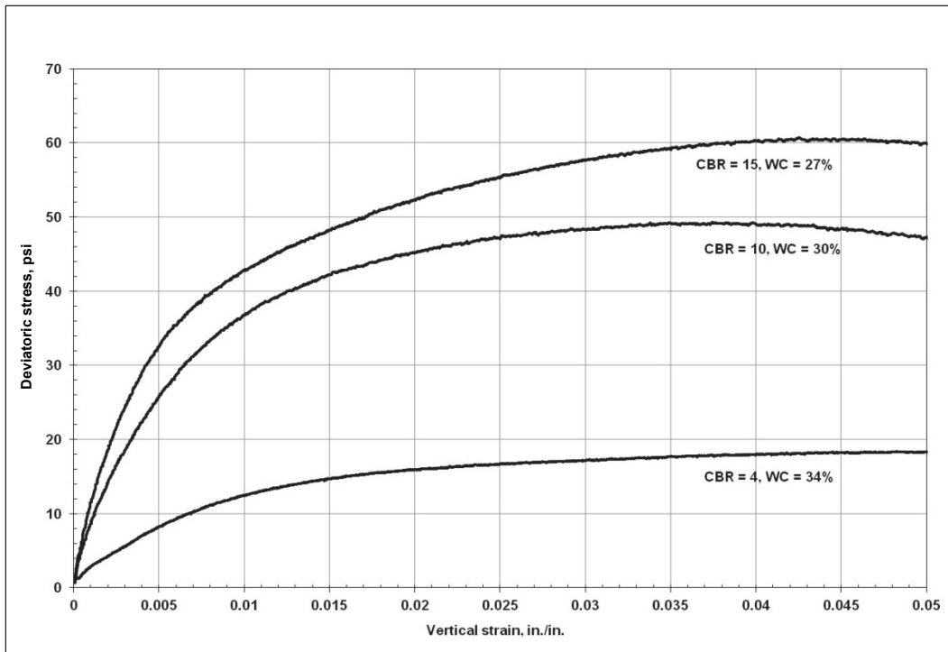
Figure 10. Stress-strain data from confined, drained triaxial compression tests on the subgrade soil.
