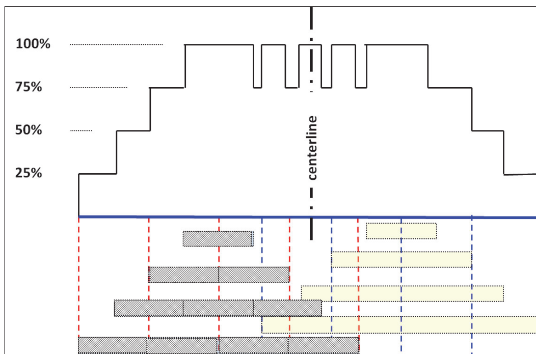
Figure 44. Traffic pattern for the C-17 dual-tire gear.
