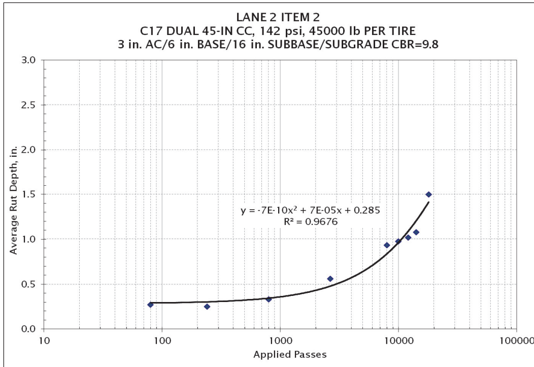
Figure 65. Rutting development on Lane 2 Item 2.
