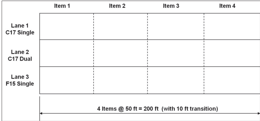
Figure 39. Section layout with traffic lane details.
