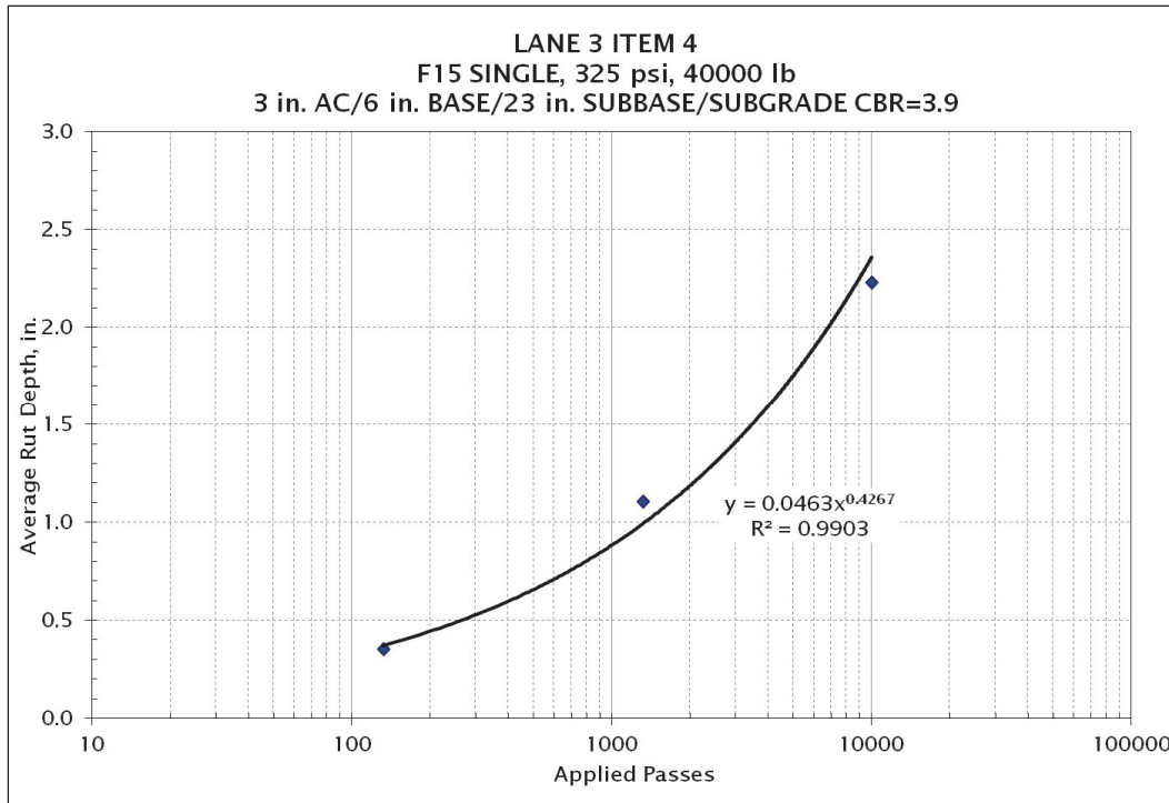
Figure 63. Rutting development on Lane 3 Item 4.
