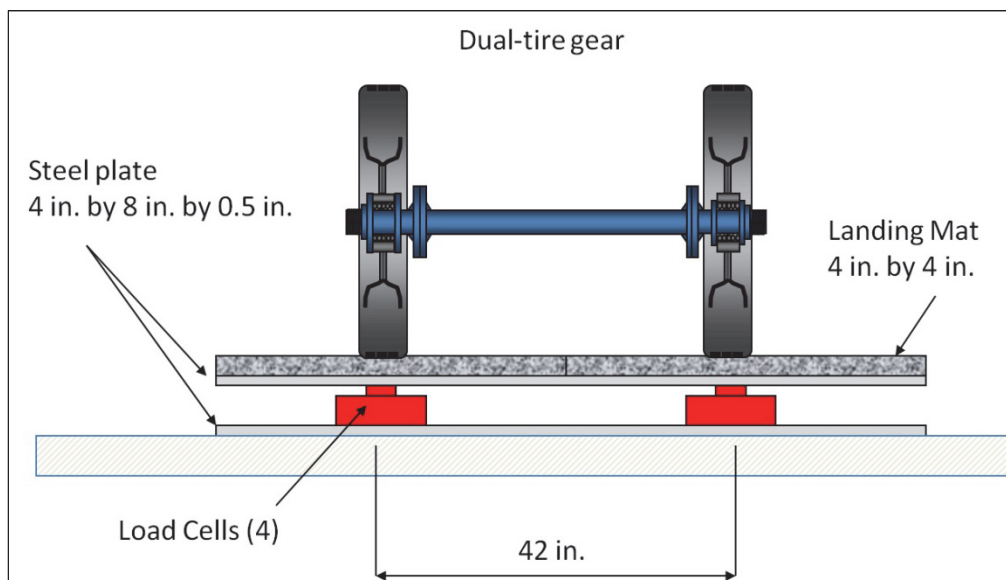
Figure 47. Calibration setup.
