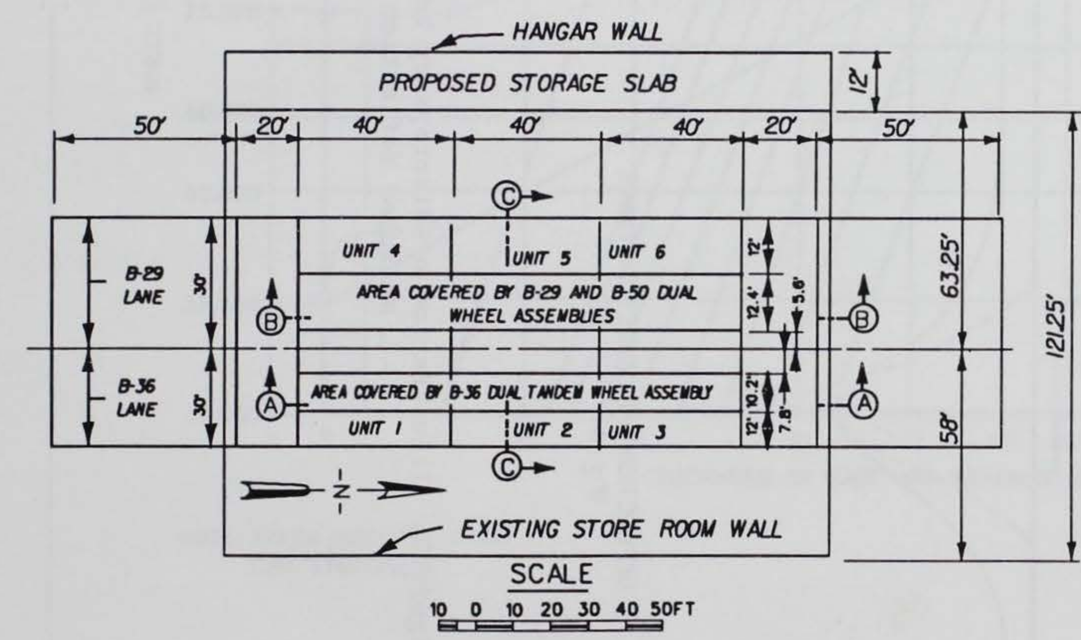
LAYOUT OF TEST LANES
