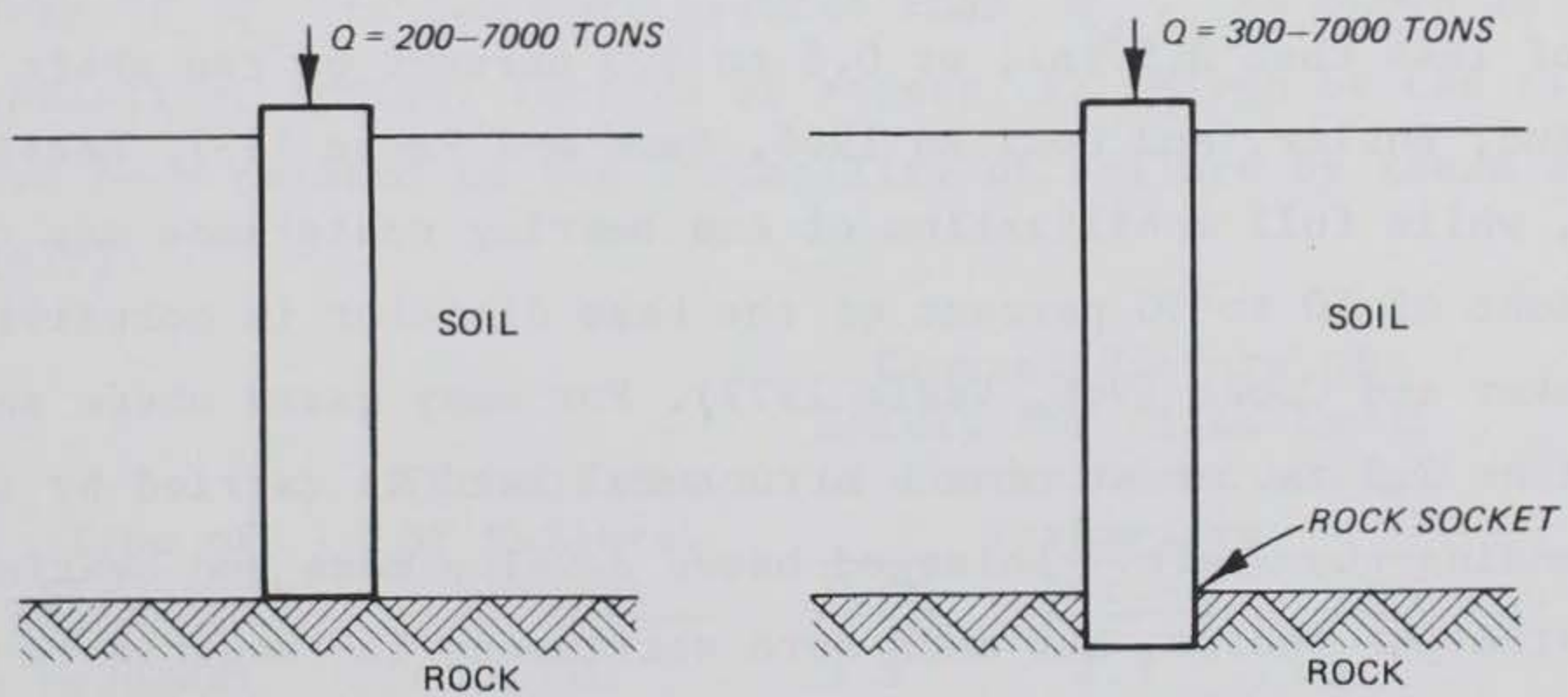
c. Shafts end bearing in rock
