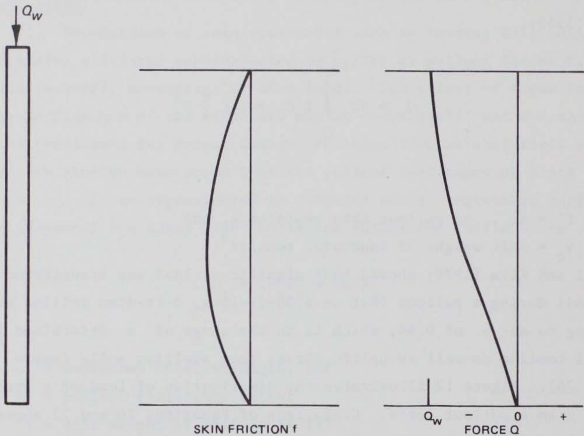
Figure 12. Distribution of load from a pullout force on a straight shaft
