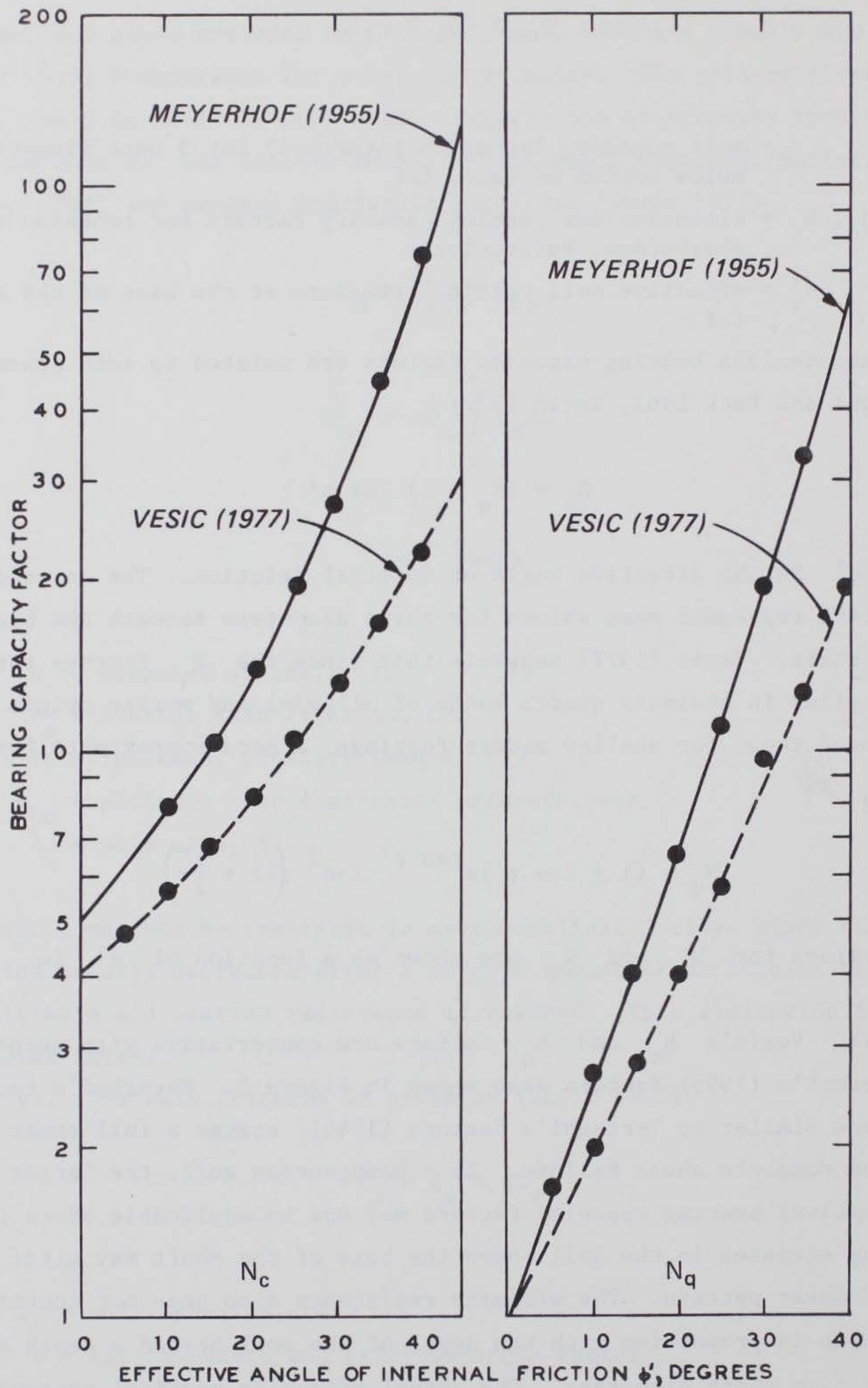
Figure 5. Bearing capacity factors N_c and N_q (Meyerhof 1955, Vesic 1977)
