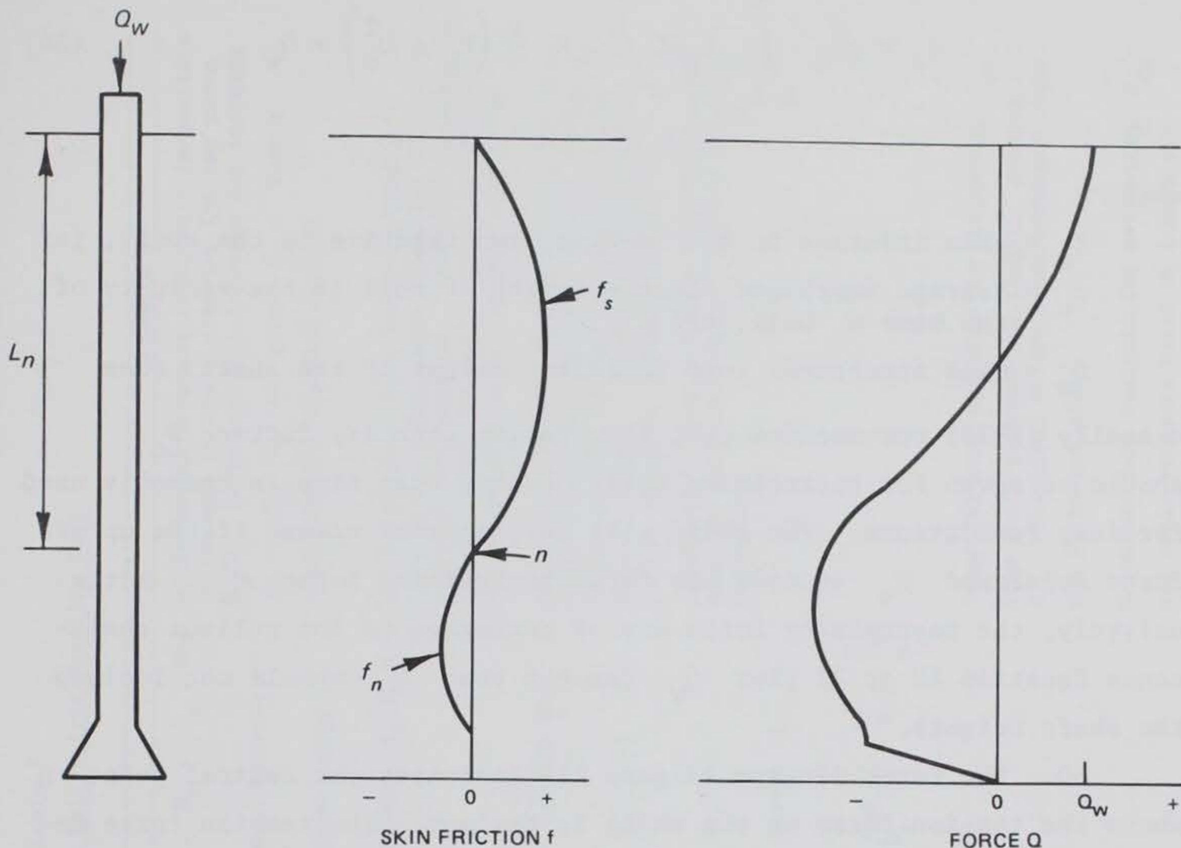
Figure 13. Distribution of load from upward thrust of swelling soil
