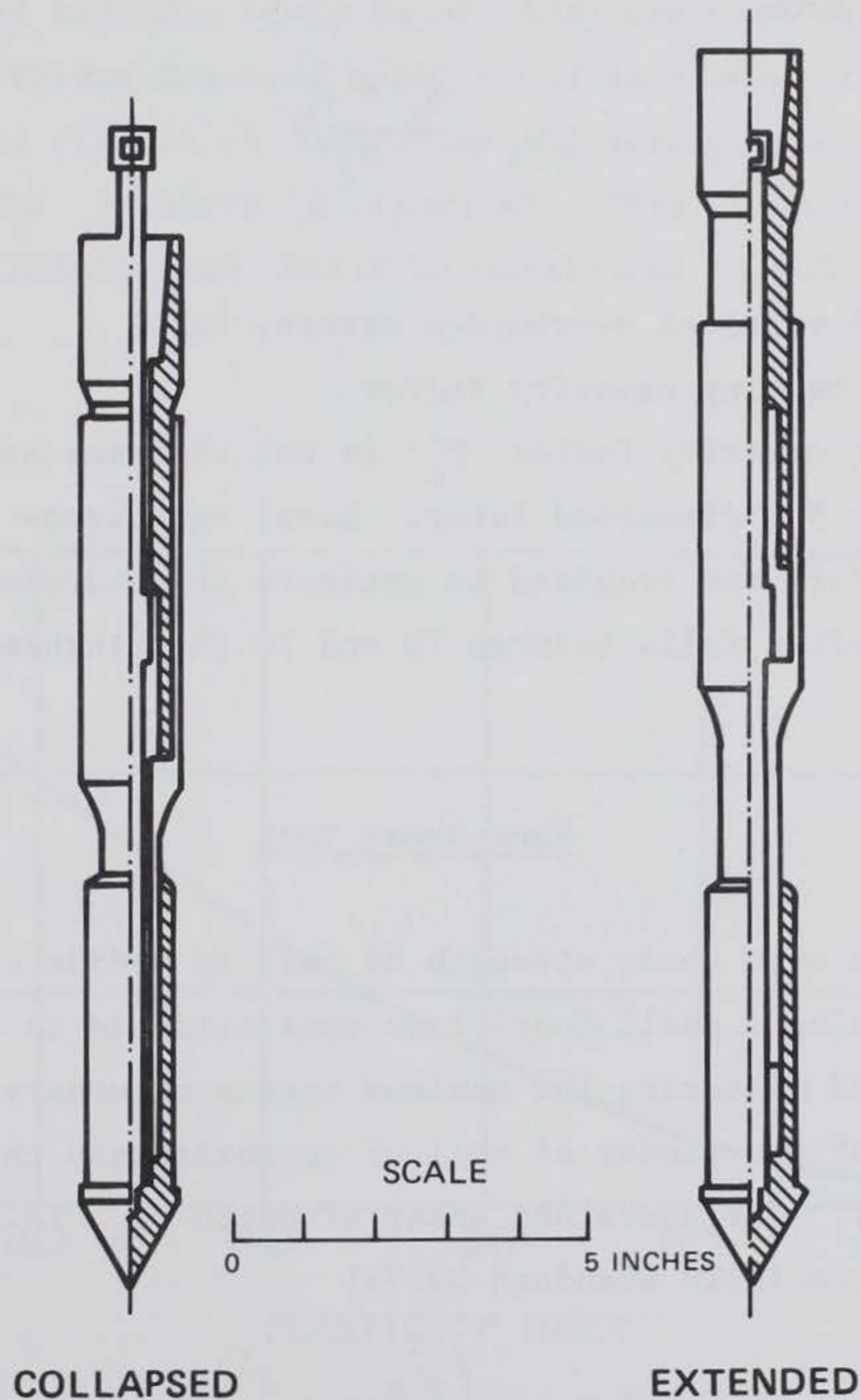
Figure A1. Example of a mechanical friction-cone penetrometer tip (Begemann Friction-cone) (after Nottingham and Grubbs 1978)
