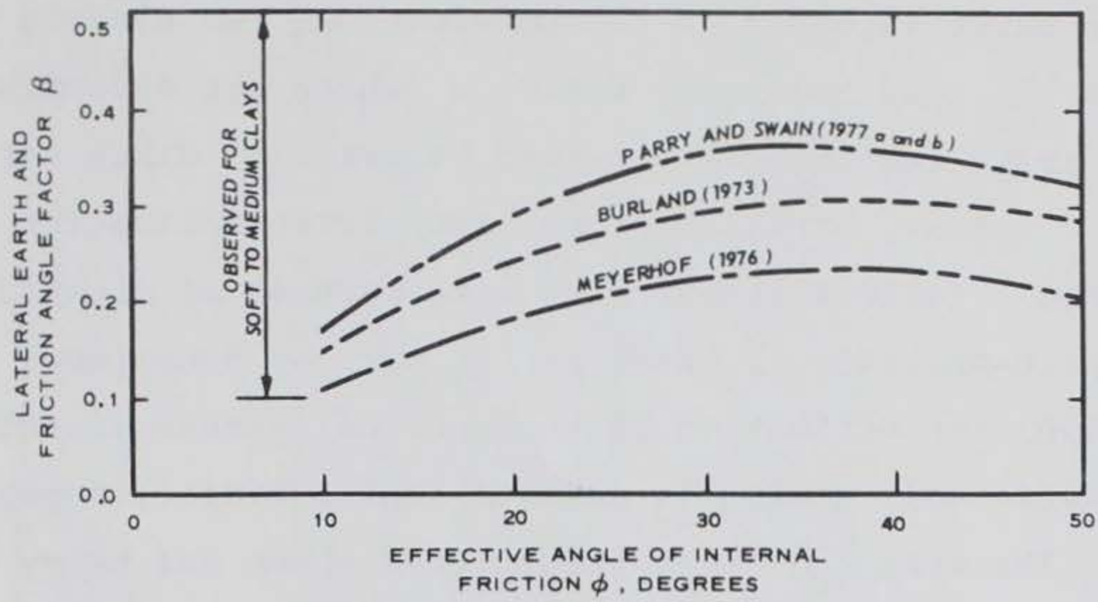
Figure 6. Comparison of methods for estimating \beta in soft to medium clays ( OCR = K_0 = 1 )
