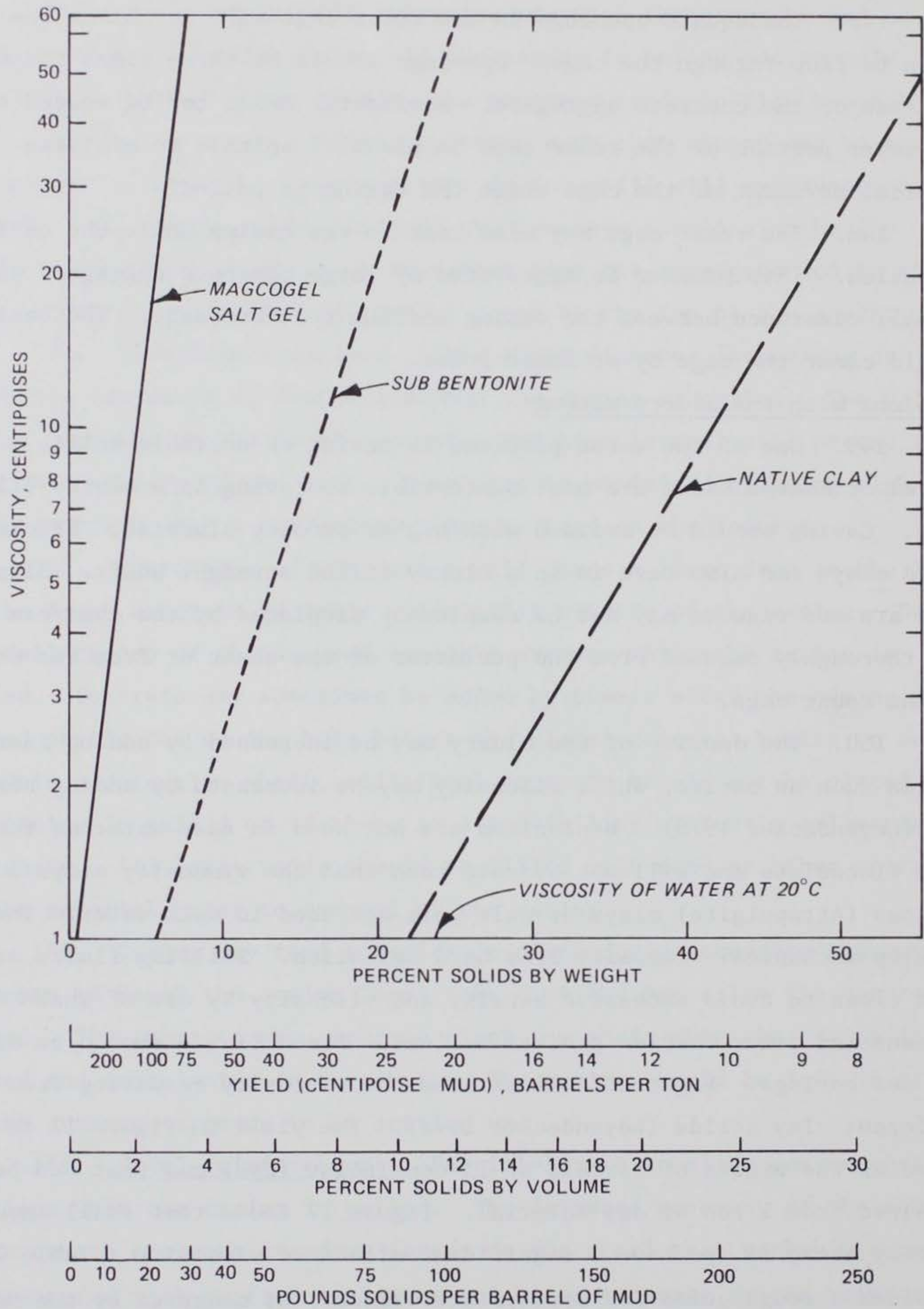
Figure 17. Viscosity curves resulting from different clay solids (adapted from Leyendecker 1978)
