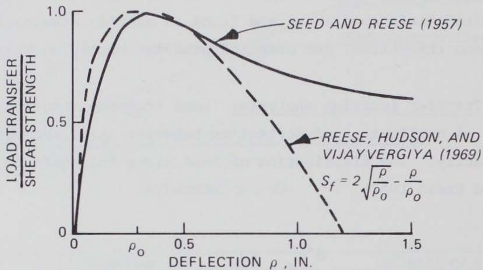
a. Transfer function for stiff clay
