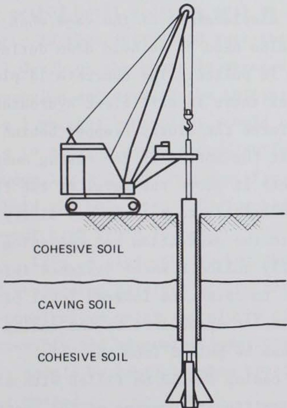
c. UNDERREAMING WITH THE CASING METHOD
