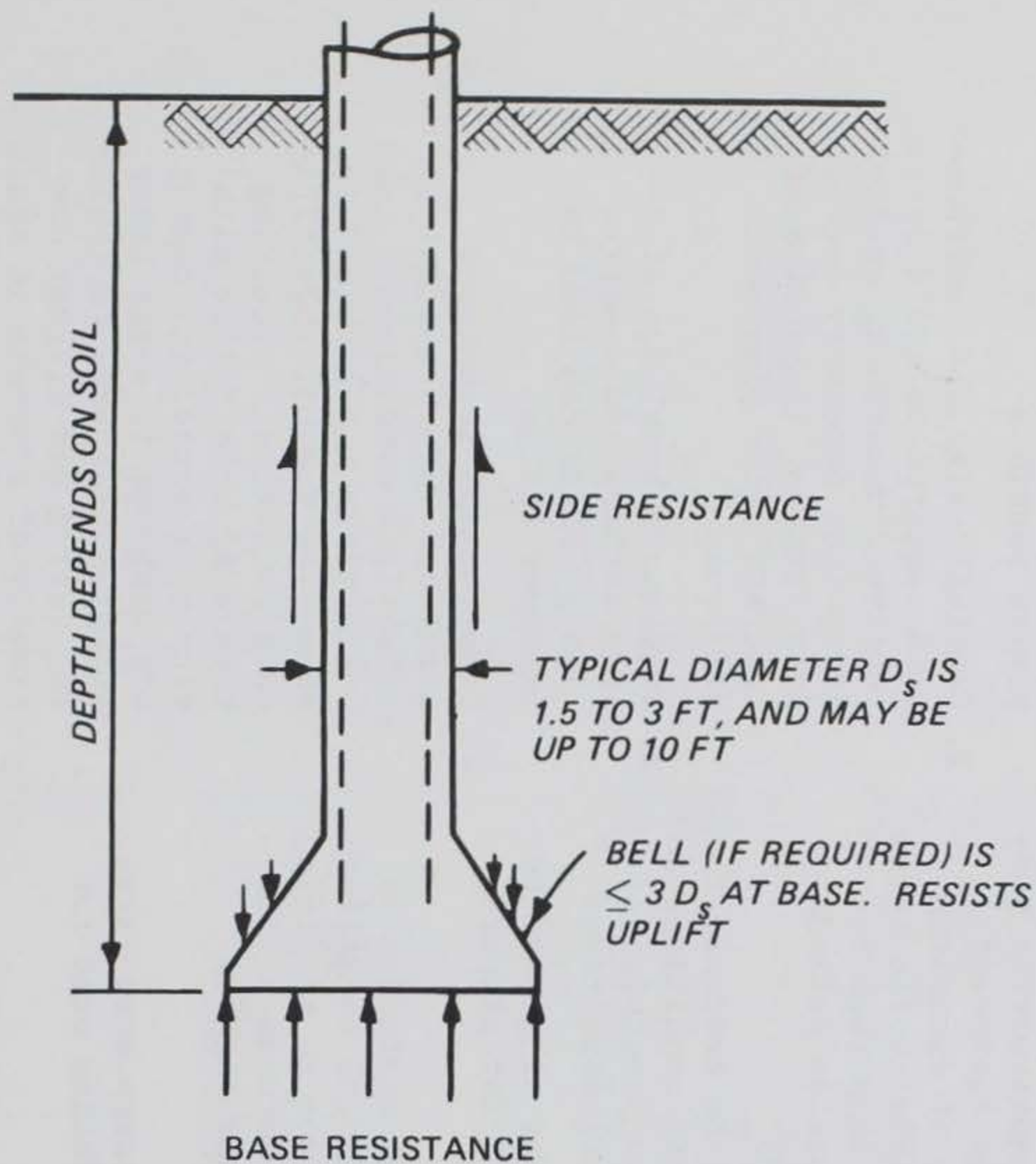
Figure 1. Typical drilled shaft
