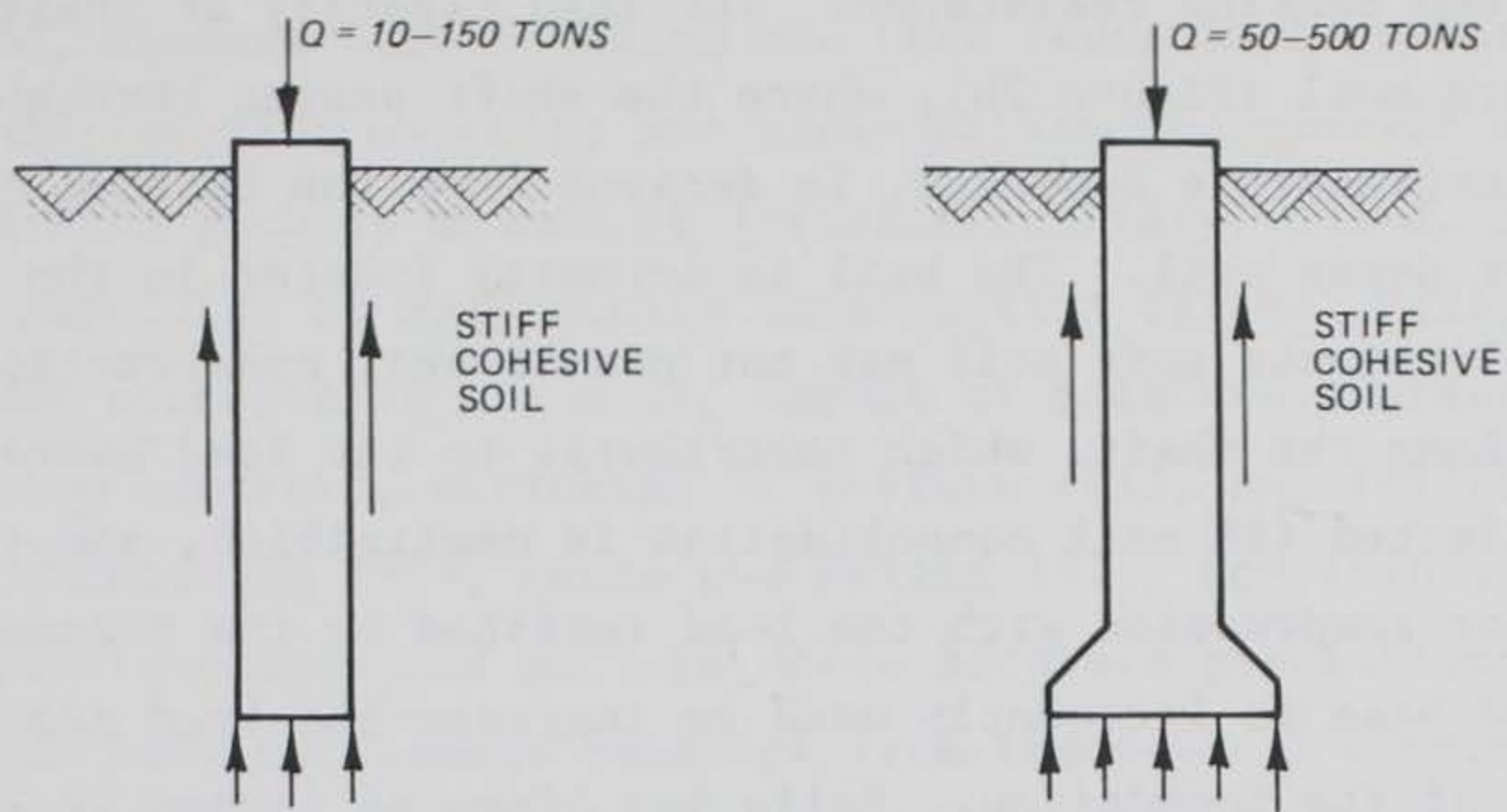
a. Floating shafts in homogeneous soil
