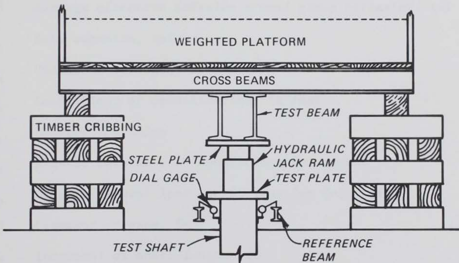
b. With weighted platform
