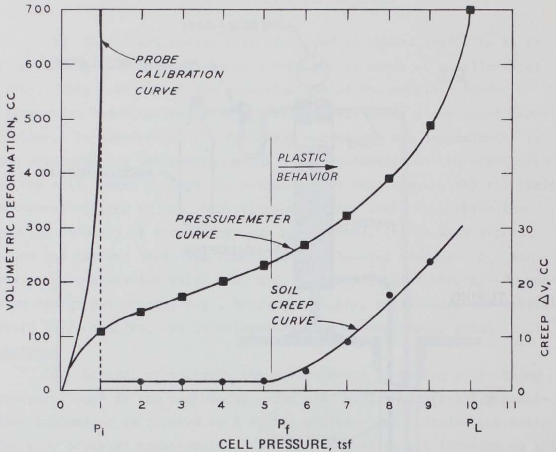
Figure A4. Typical pressuremeter and creep curves (after Canadian Geotechnical Society 1979)
