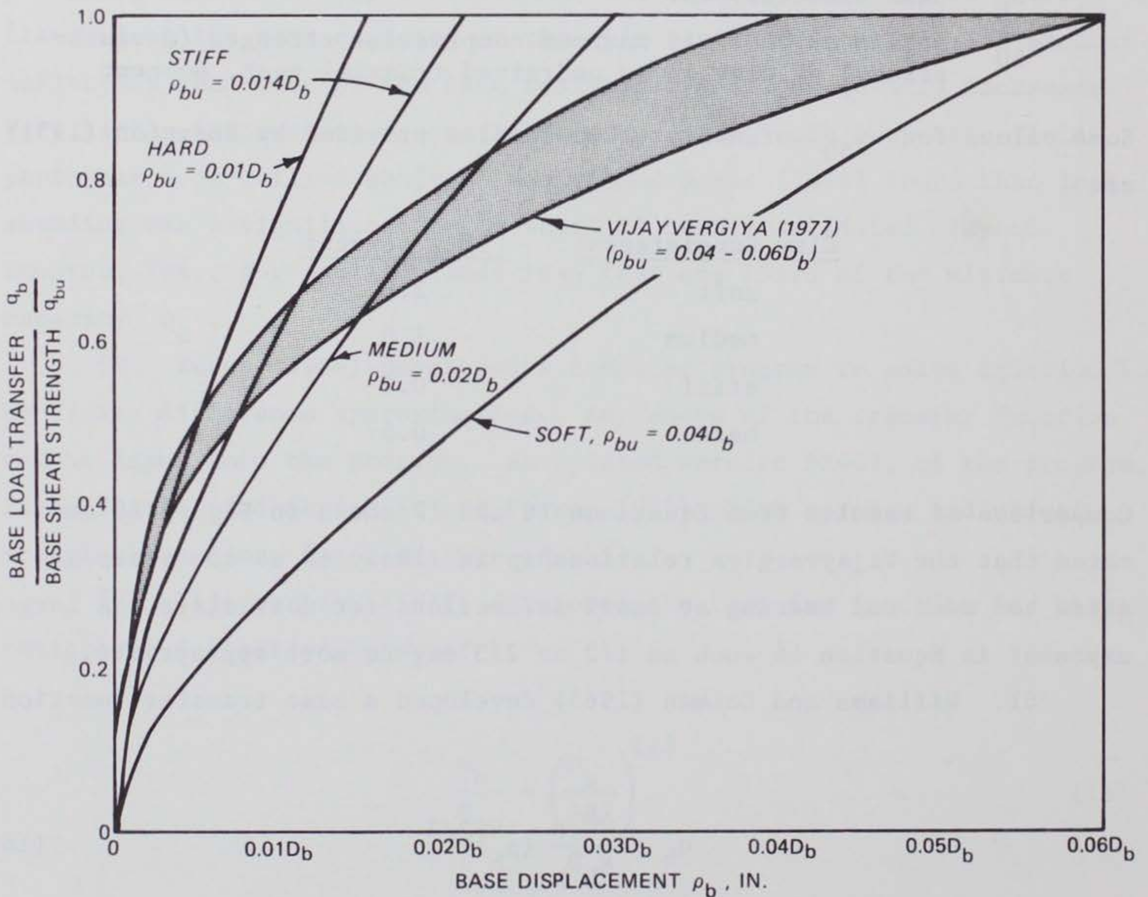
Figure 10. Comparison of base load transfer relationships
