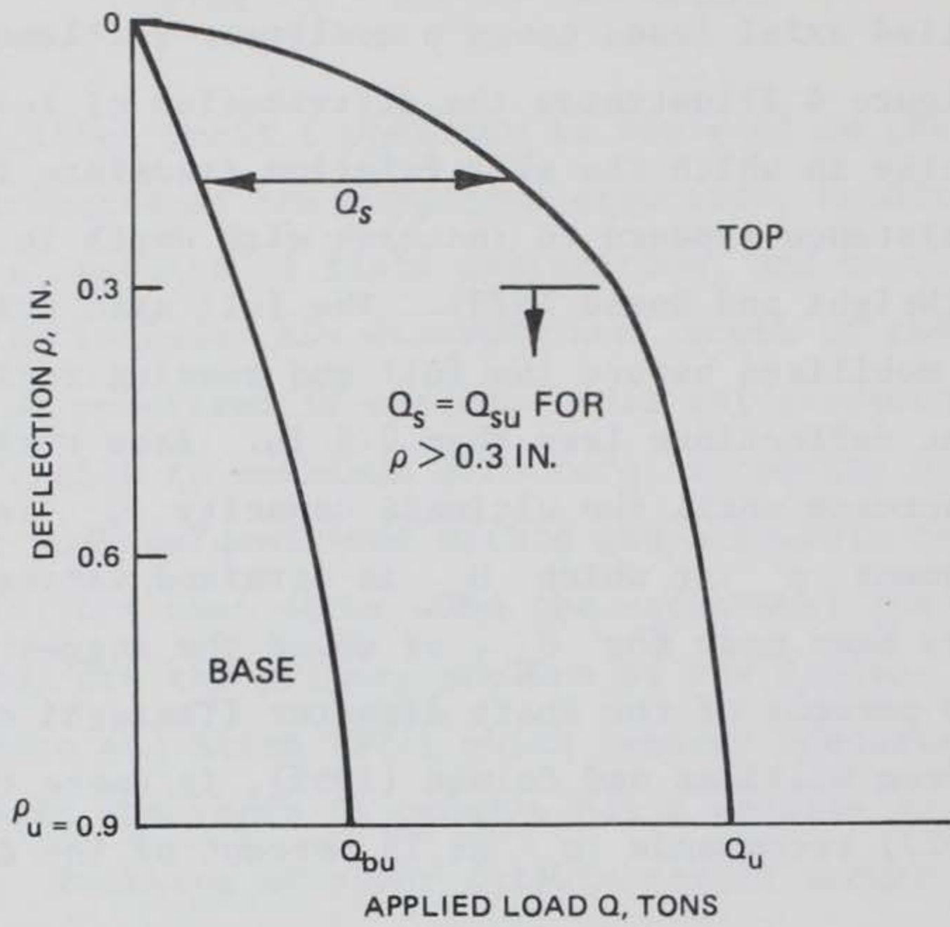
Figure 3. Axial load-deflection relationship
