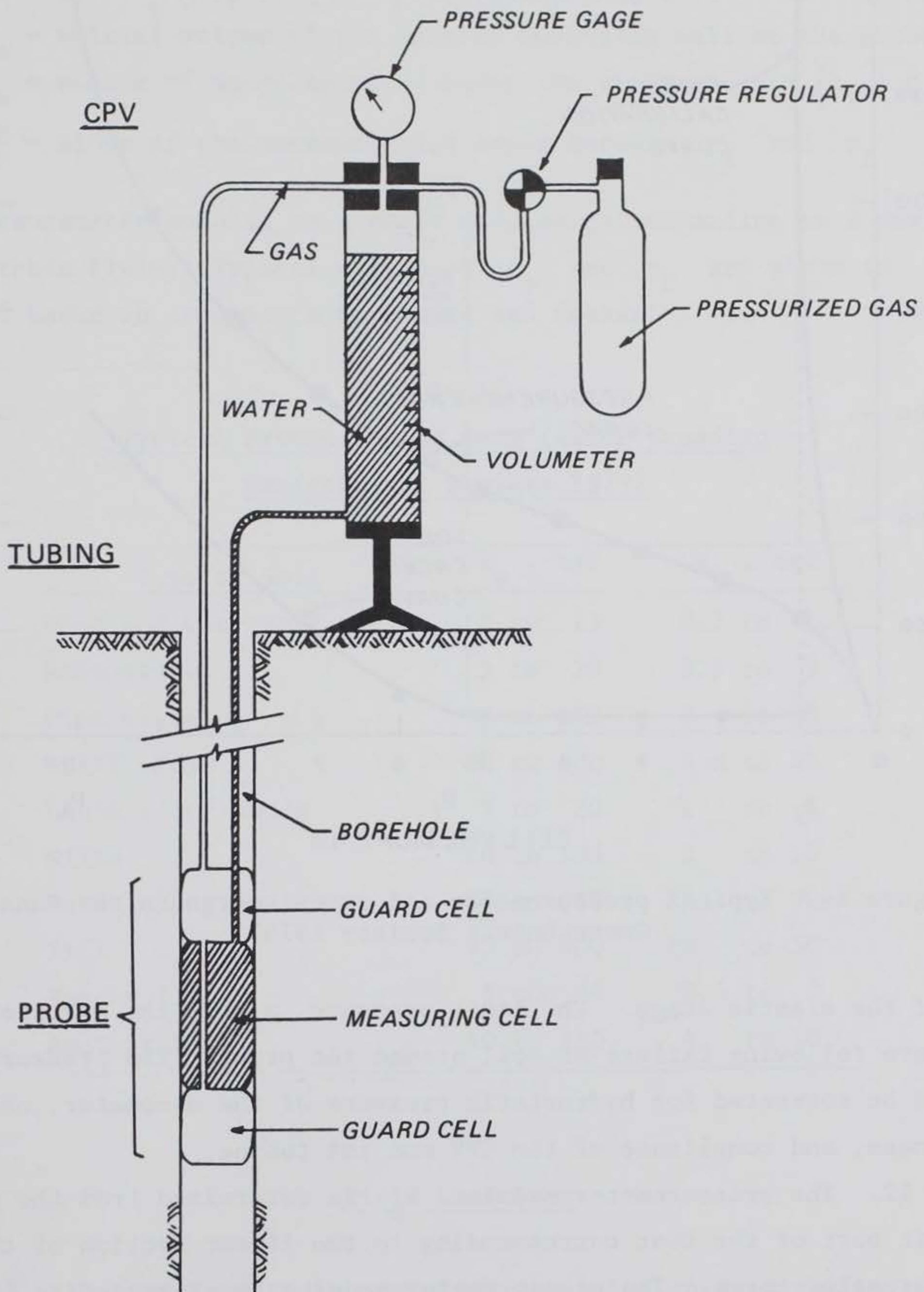
Figure A3. Schematic view of a pressuremeter sketch showing the CPV and probe (after Canadian Geotechnical Society 1979)
