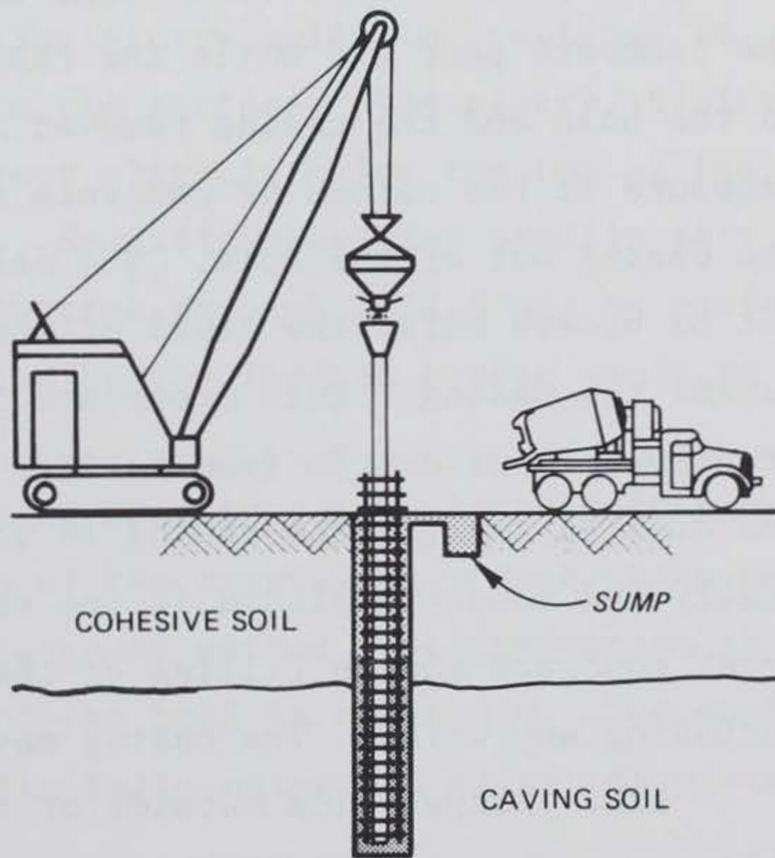
d. PLACING CONCRETE USING A TREMIE AND THE SLURRY METHOD
