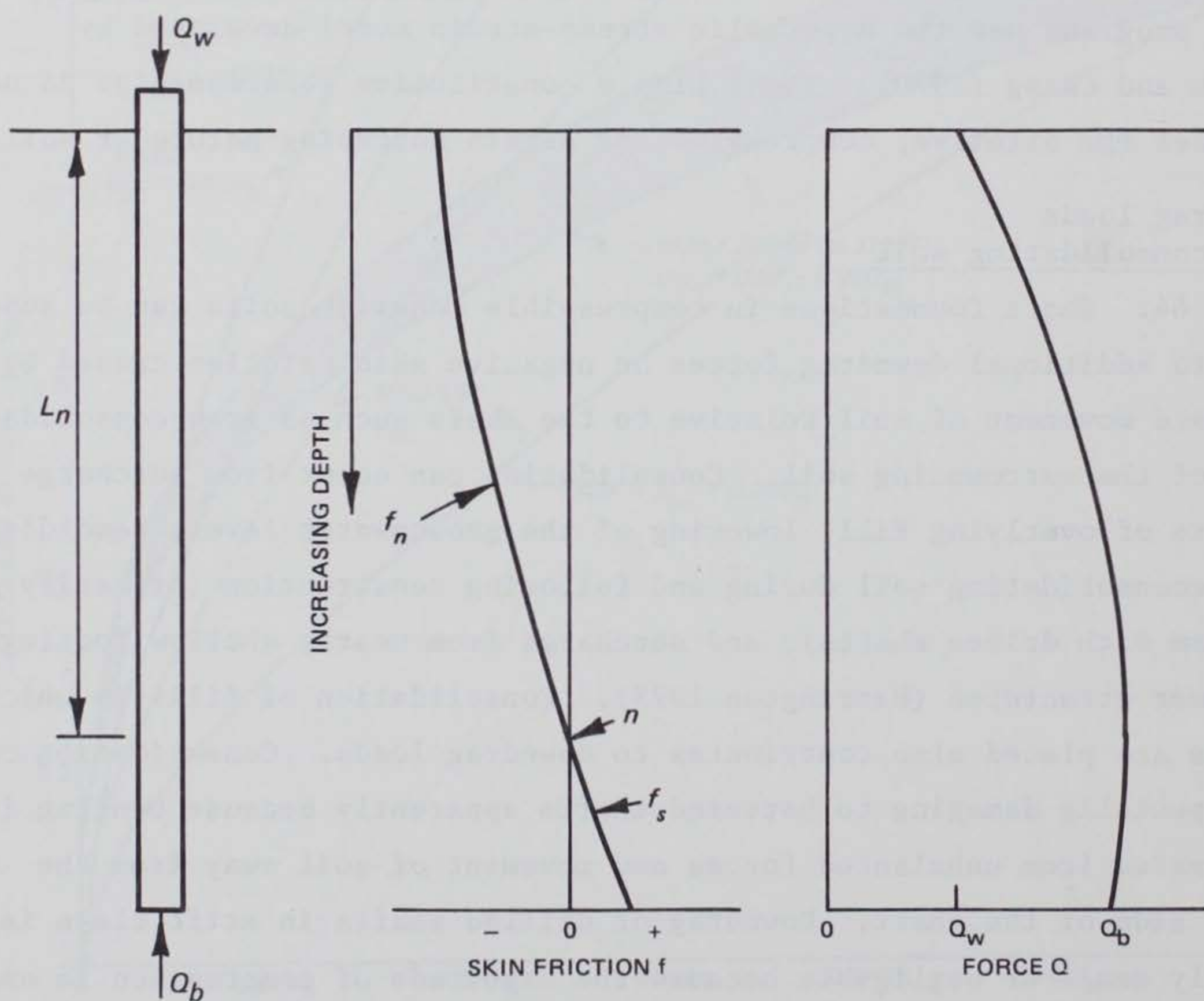
Figure 11. Distribution of load from negative skin friction
