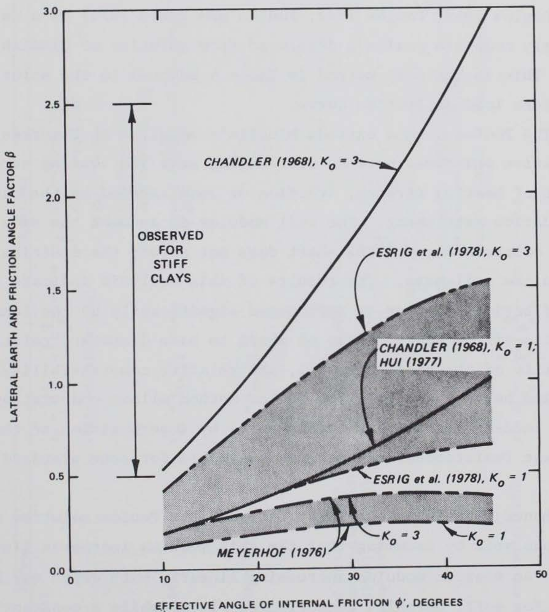
Figure 7. Comparison of methods for estimating \beta in stiff clays
