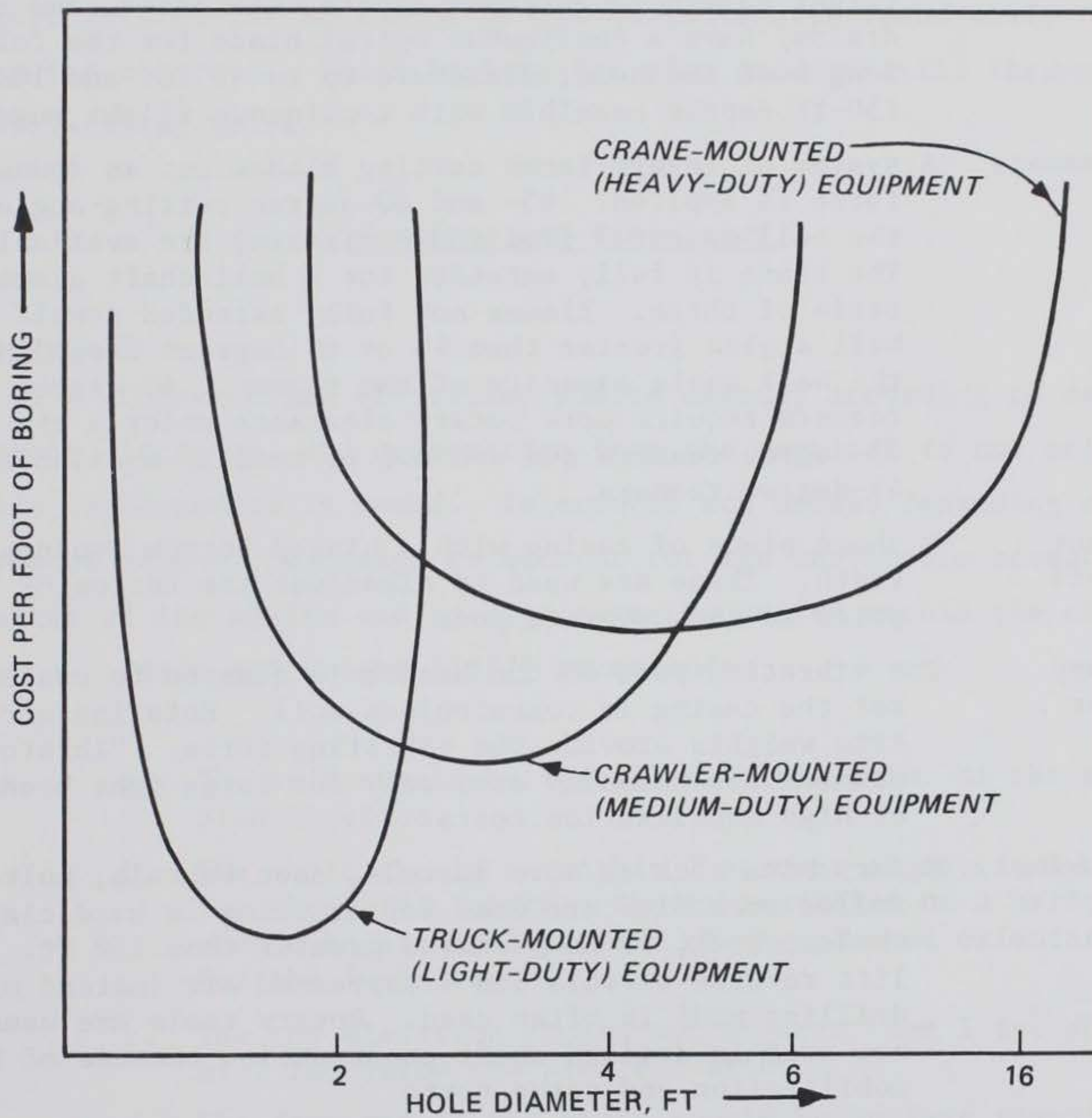
Figure 15. Relative costs for different drilling equipment (After Drilled Pier Foundation , by Woodward, Gardner, and Greer. Copyright © 1972 by McGraw Hill, Inc. Used with the permission of McGraw-Hill Book Company)
