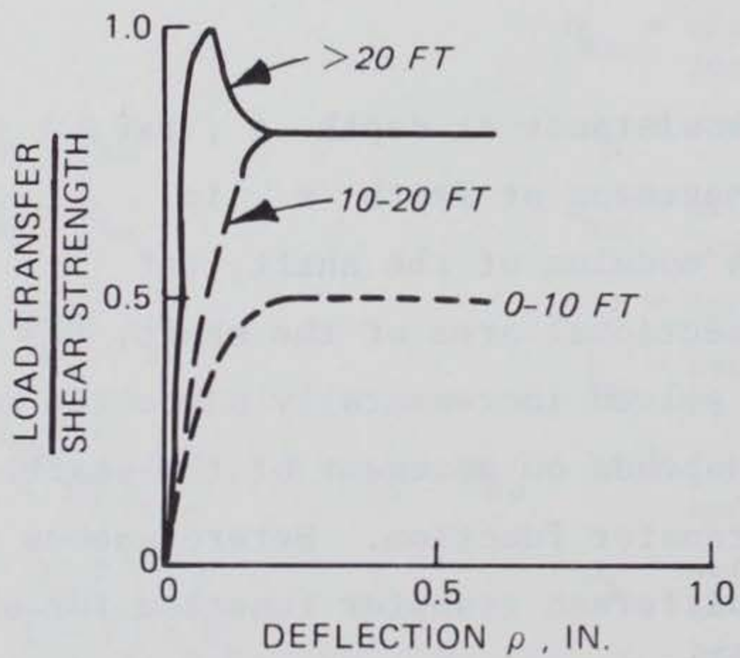
b. Transfer function with depth (Coyle and Reese 1966)
