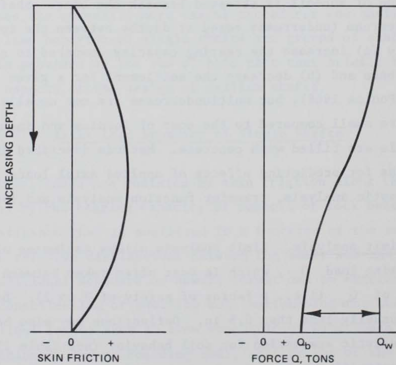
Figure 4. Distribution of axial load with depth
