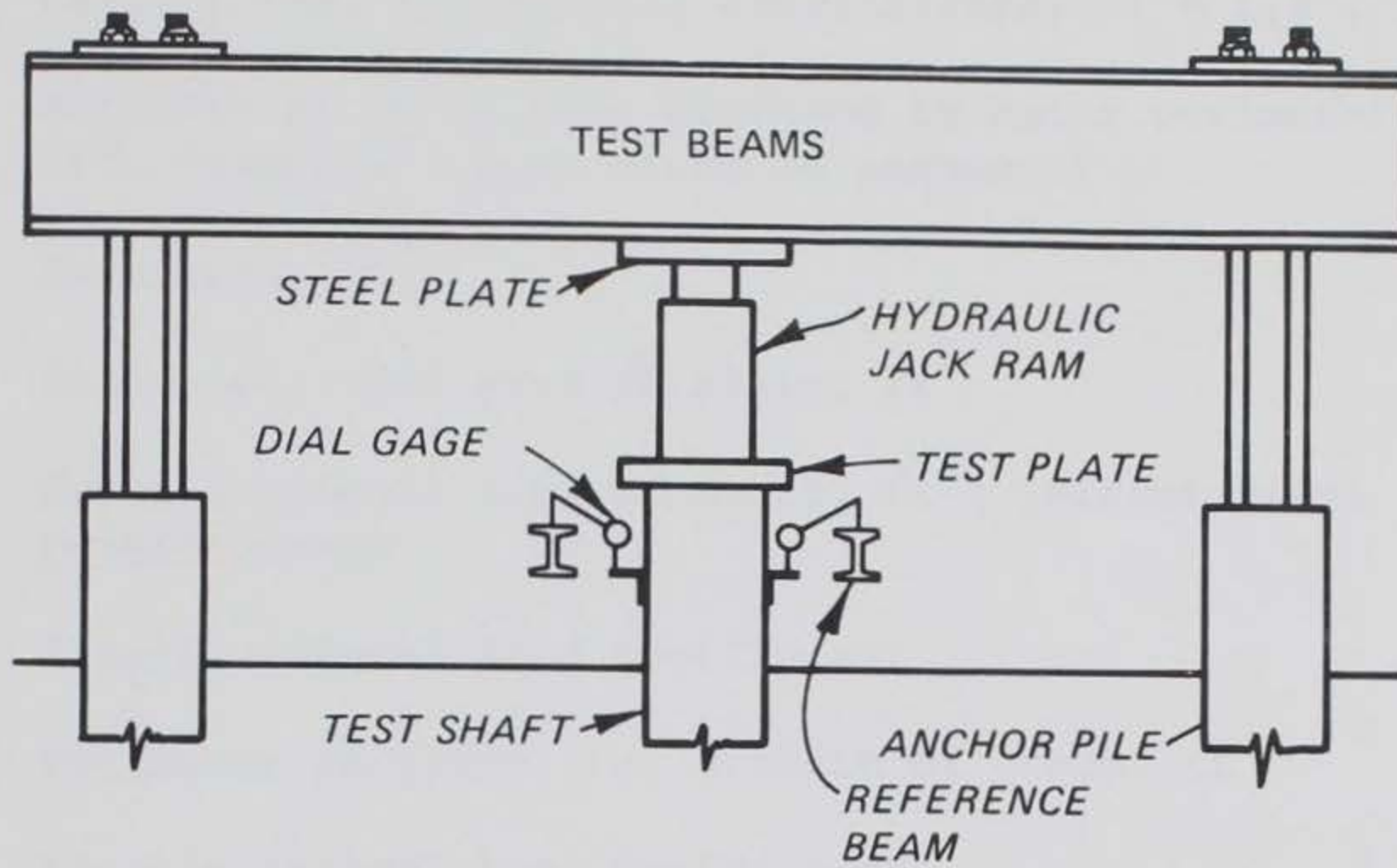
a. With anchored piles
