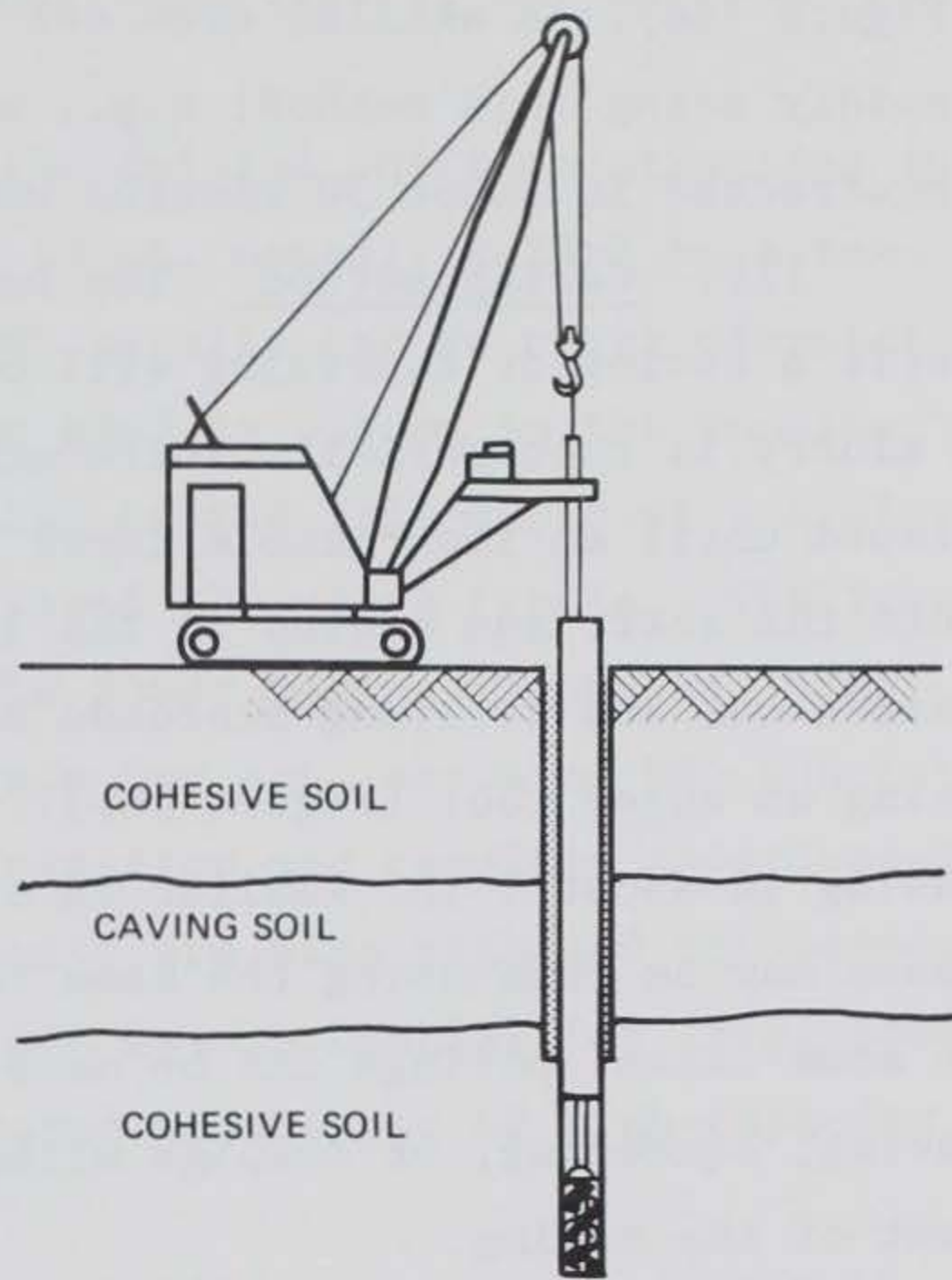
b. DRILLING WITH THE CASING METHOD
