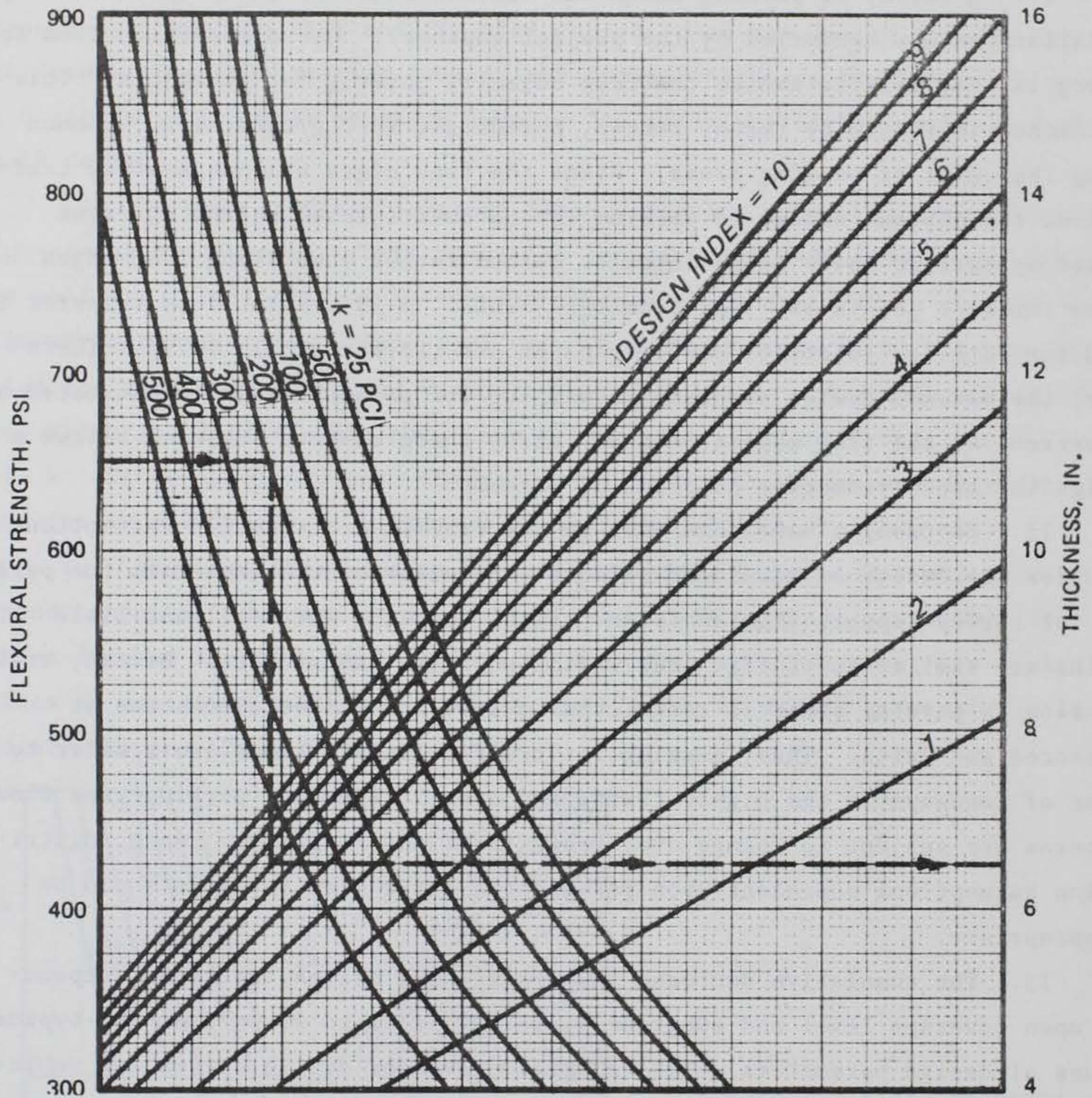
Figure 2. Rigid pavement design curves for parking areas
