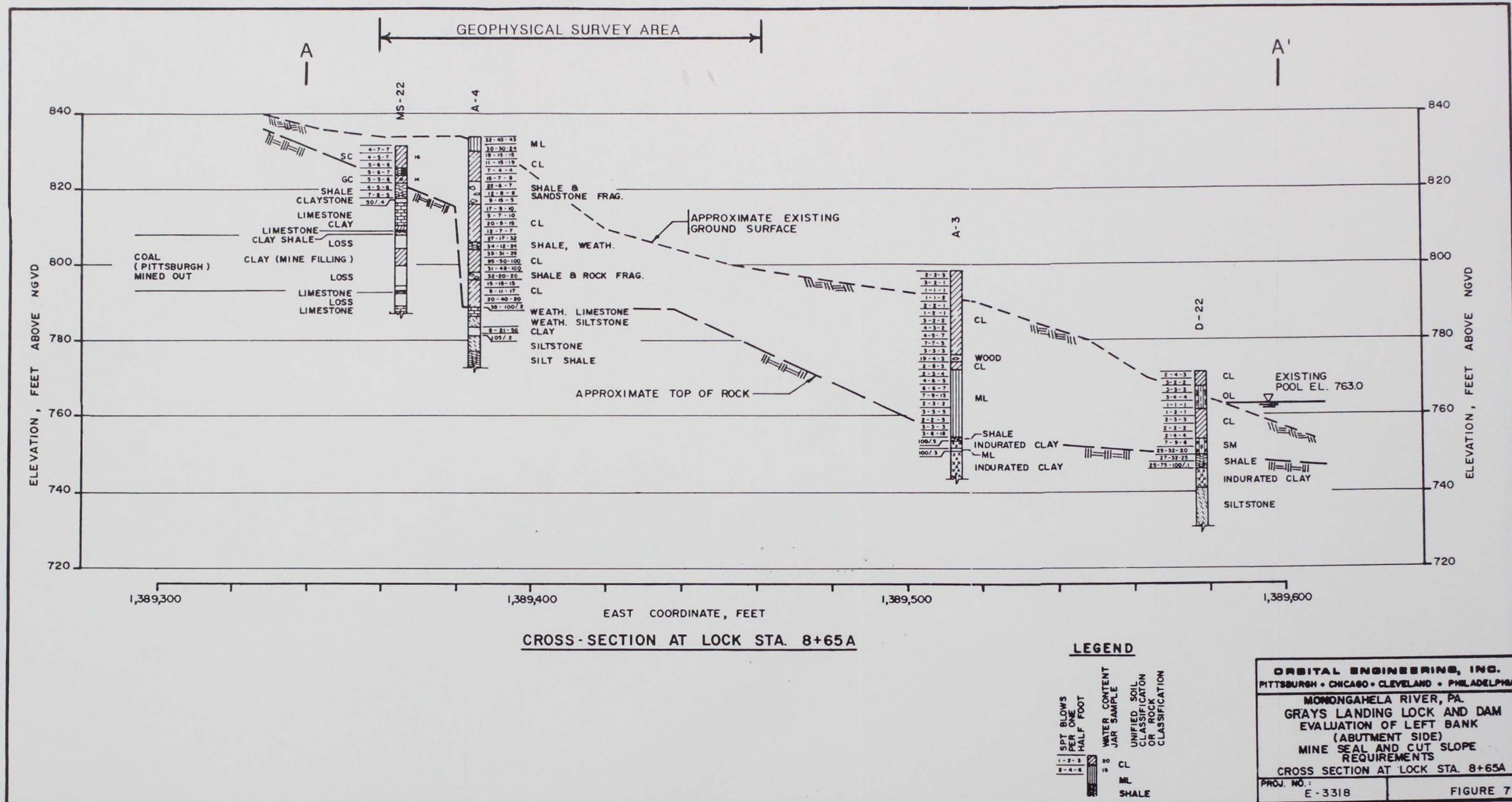
Figure 1b. Cross-section AA'.
