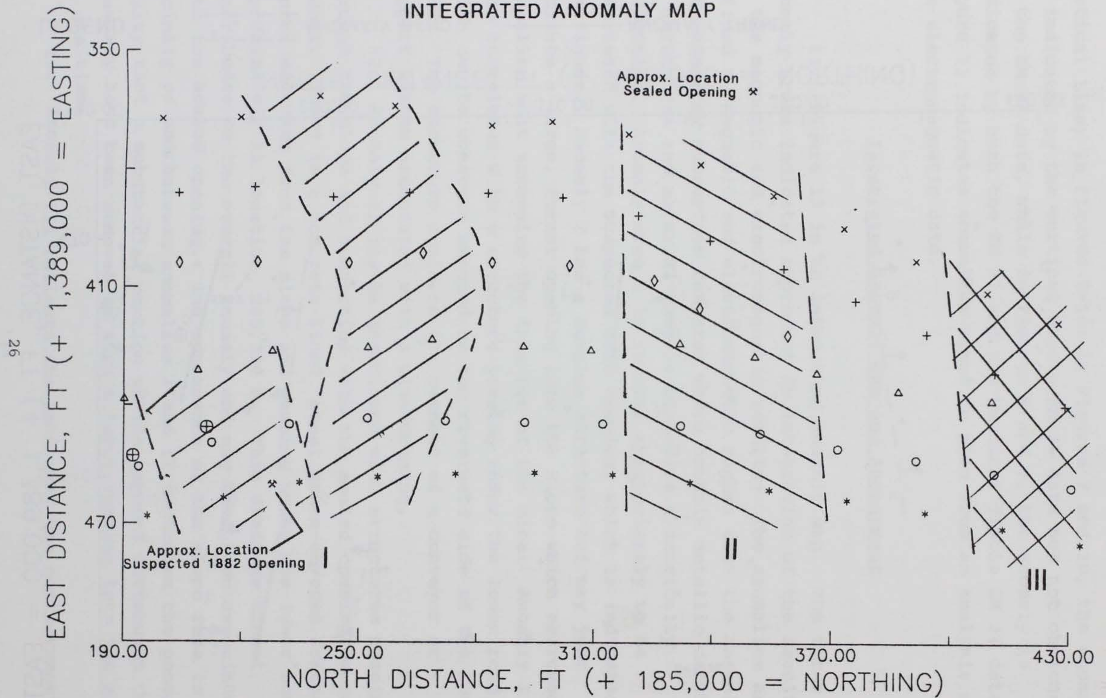
Figure 13. Integrated anomaly map for a portion of the left abutment area of Grays Landing Lock and Dam Site
