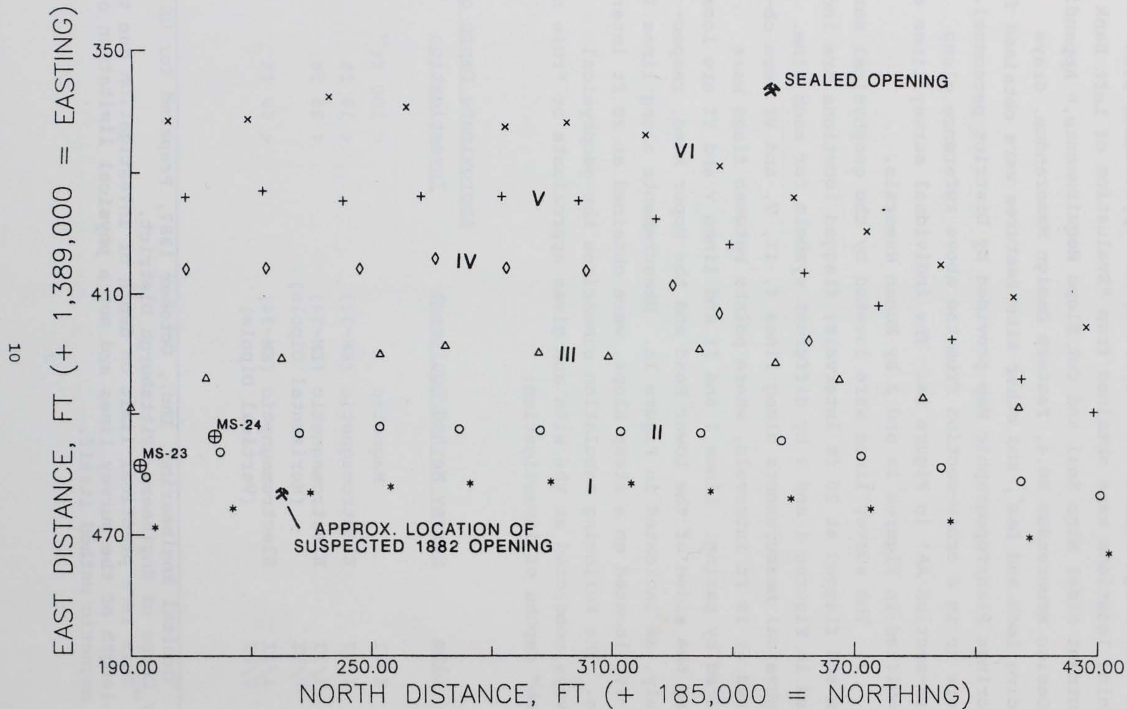
Figure 2. Geophysical survey lines, designated by Roman Numerals. Different symbols for each survey line designate flagged locations at 20 ft spacing
