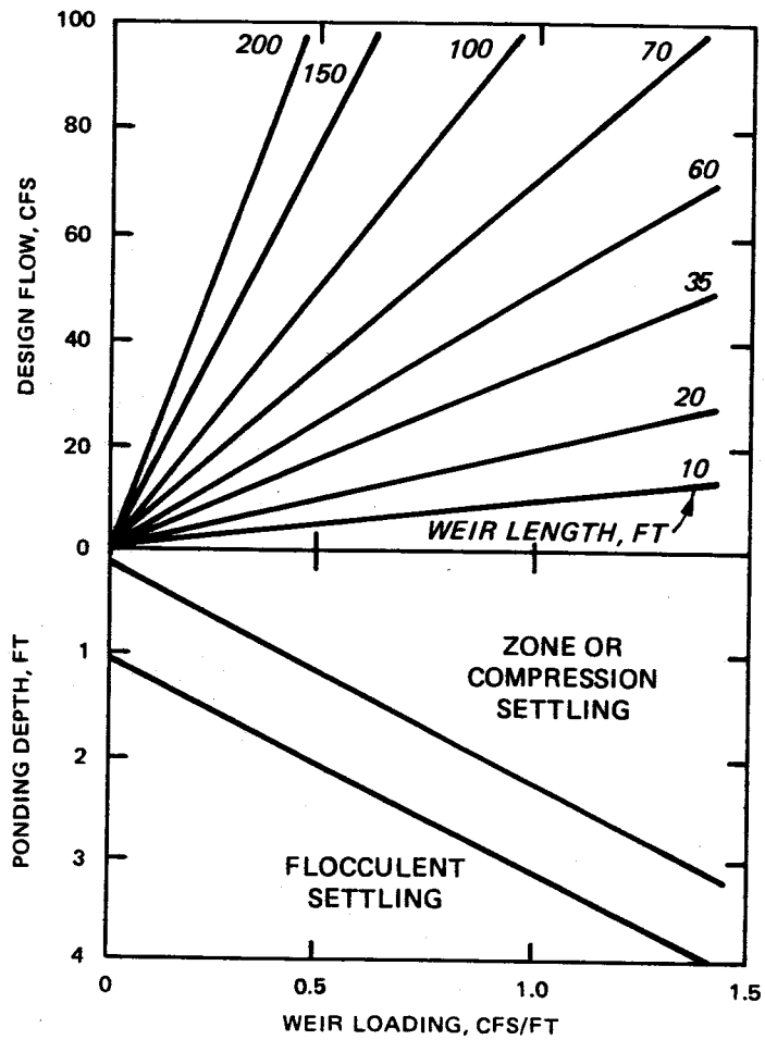
Figure 15. Weir design nomograph
