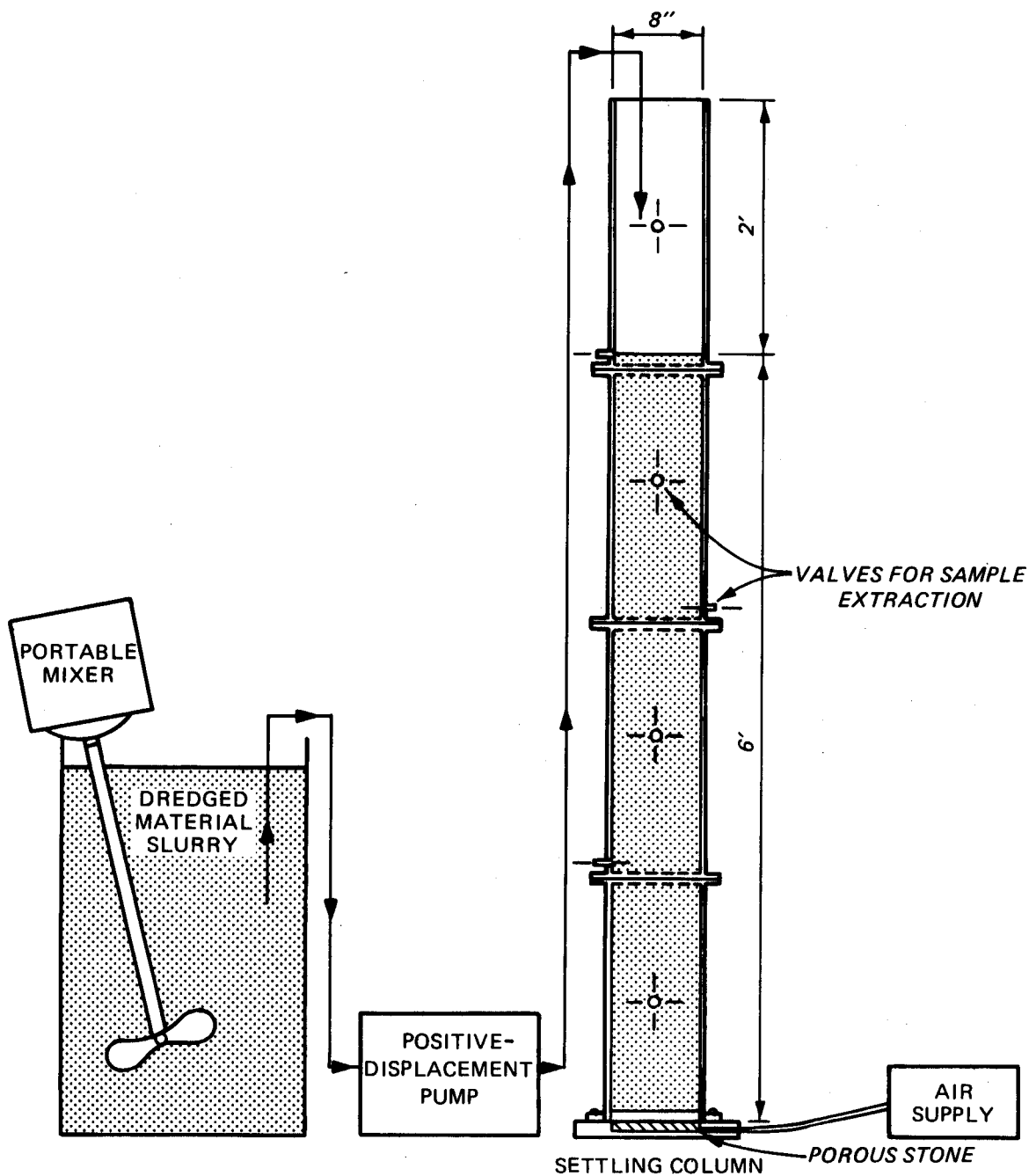
Figure 1. Schematic of the settling column
