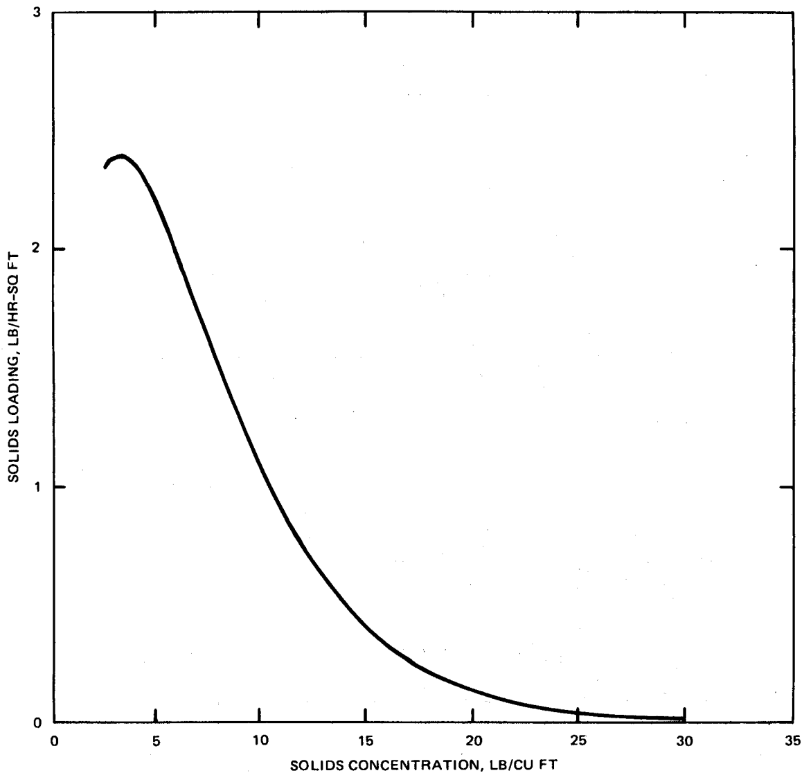
Figure 5. Solids loading curve
