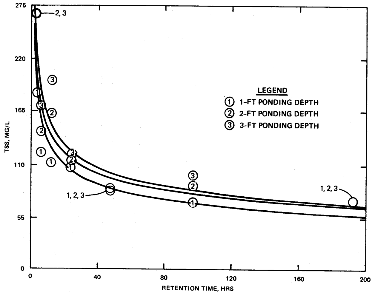
Figure 7. Composite supernatant suspended solids curve
