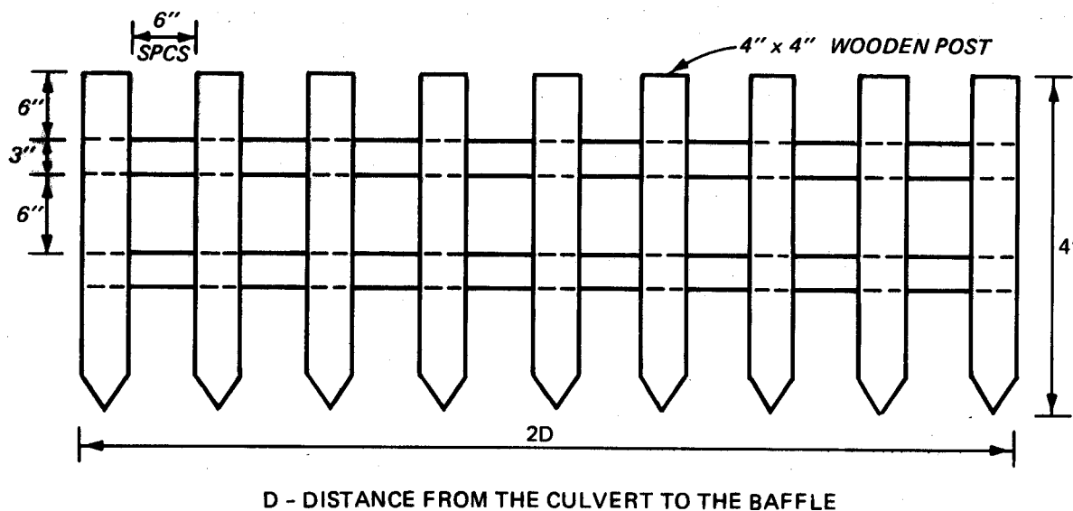
Figure 18. Slotted baffles.
