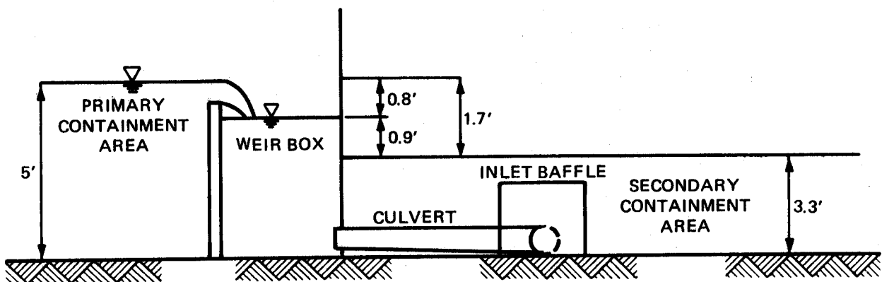
Figure 17. Weir mixing system
