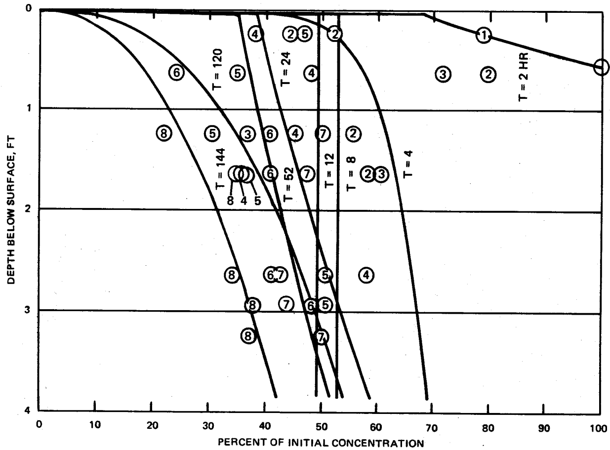
Figure 10. Capping material solids concentration profile curve
