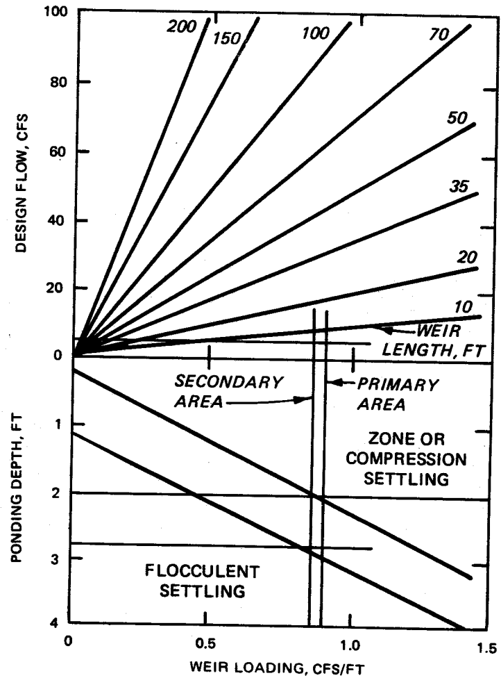
Figure 16. Example of a weir design
