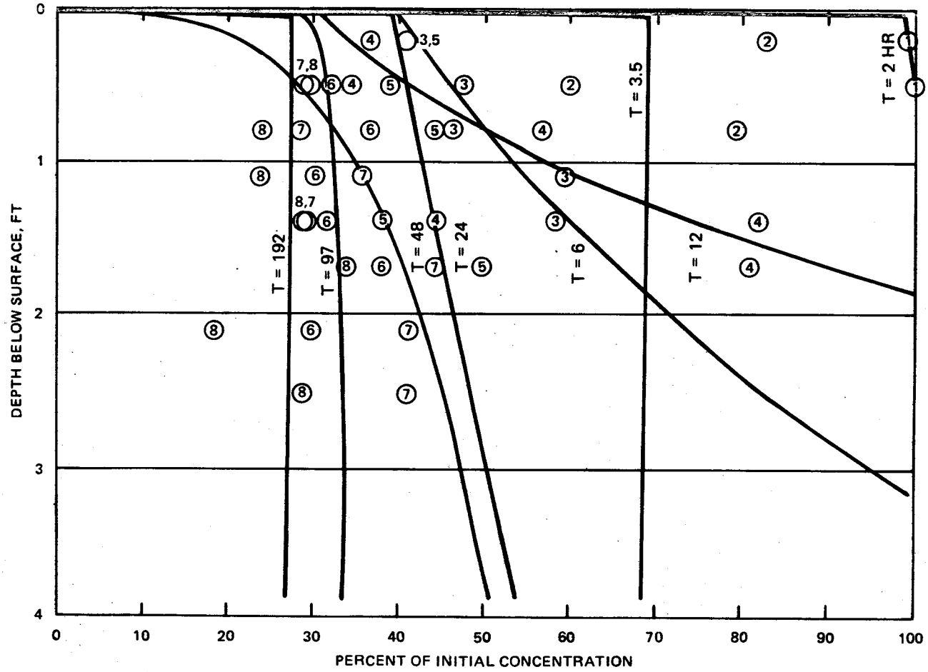
Figure 6. Composite solids concentration profile curve
