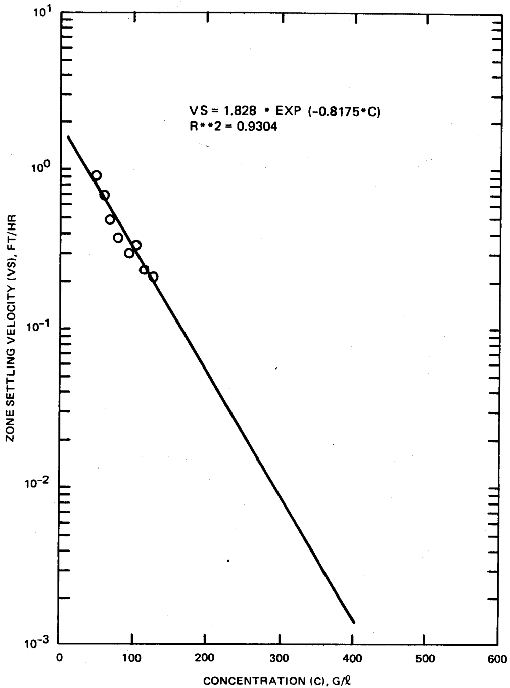
Figure 4. Zone settling curve
