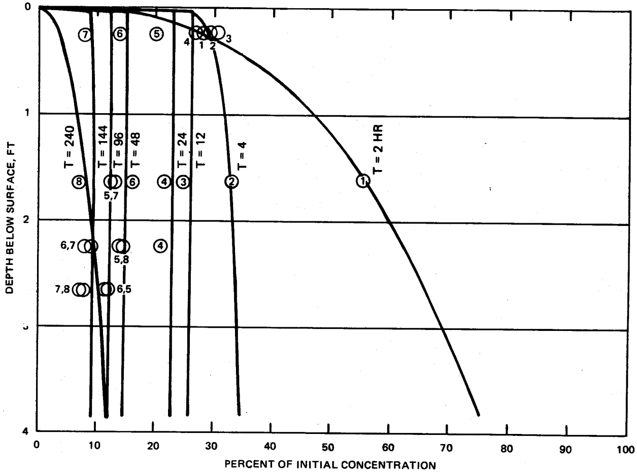
Figure 8. Hot spot solids concentration profile curve
