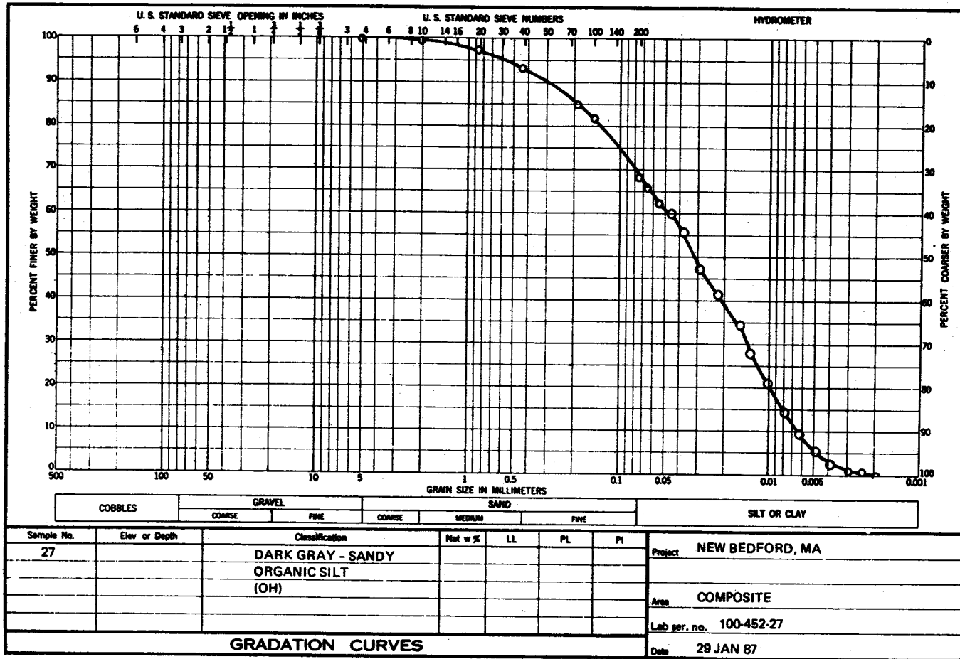
Figure 14. Grain size distribution curve
