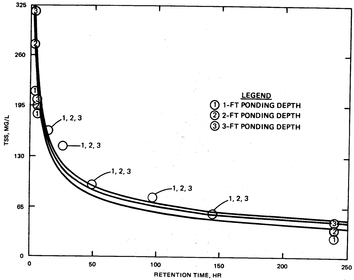
Figure 9. Hot spot supernatant suspended solids curve
