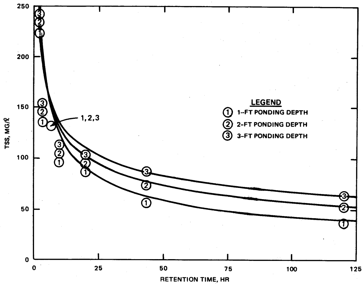
Figure 11. Capping material supernatant suspended solids curve
