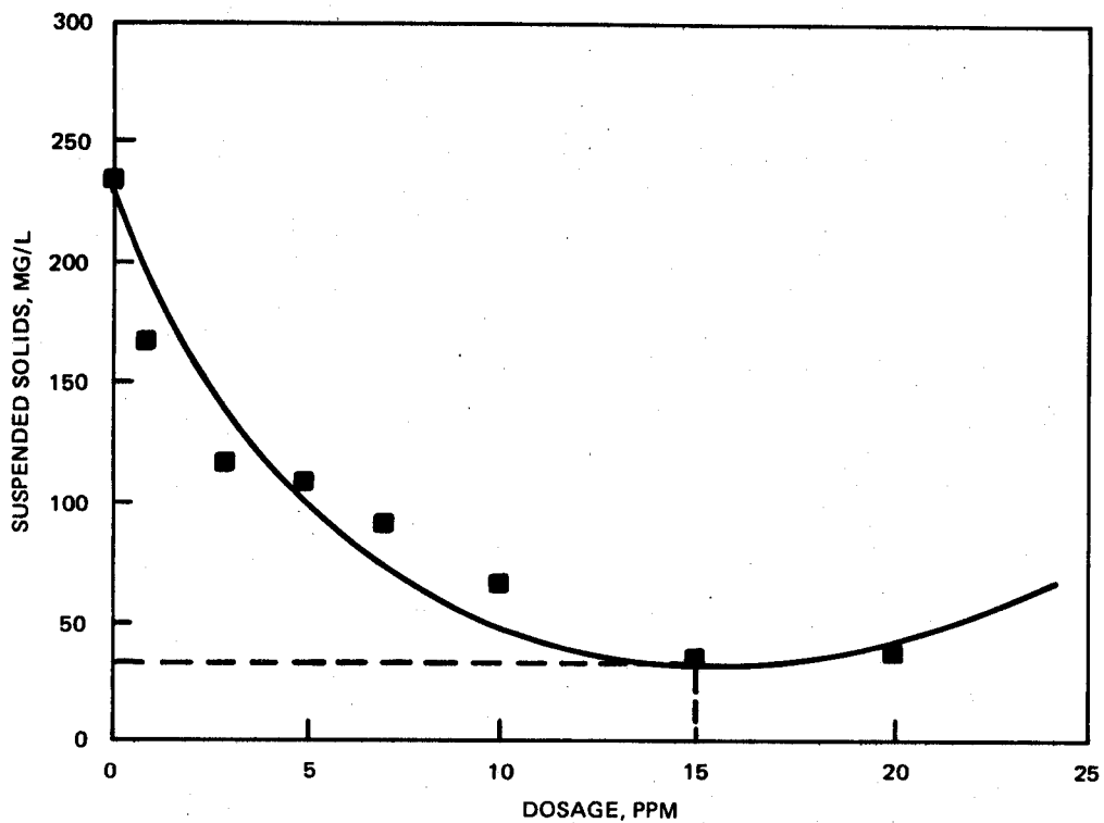
Figure 13. Polymer optimum dosage curve, Magnifloc 1586C
