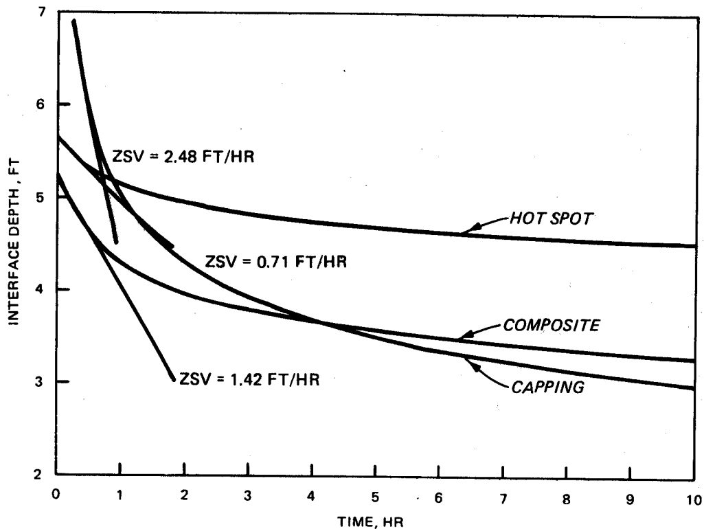
Figure 3. Comparison of the interface depth versus time
